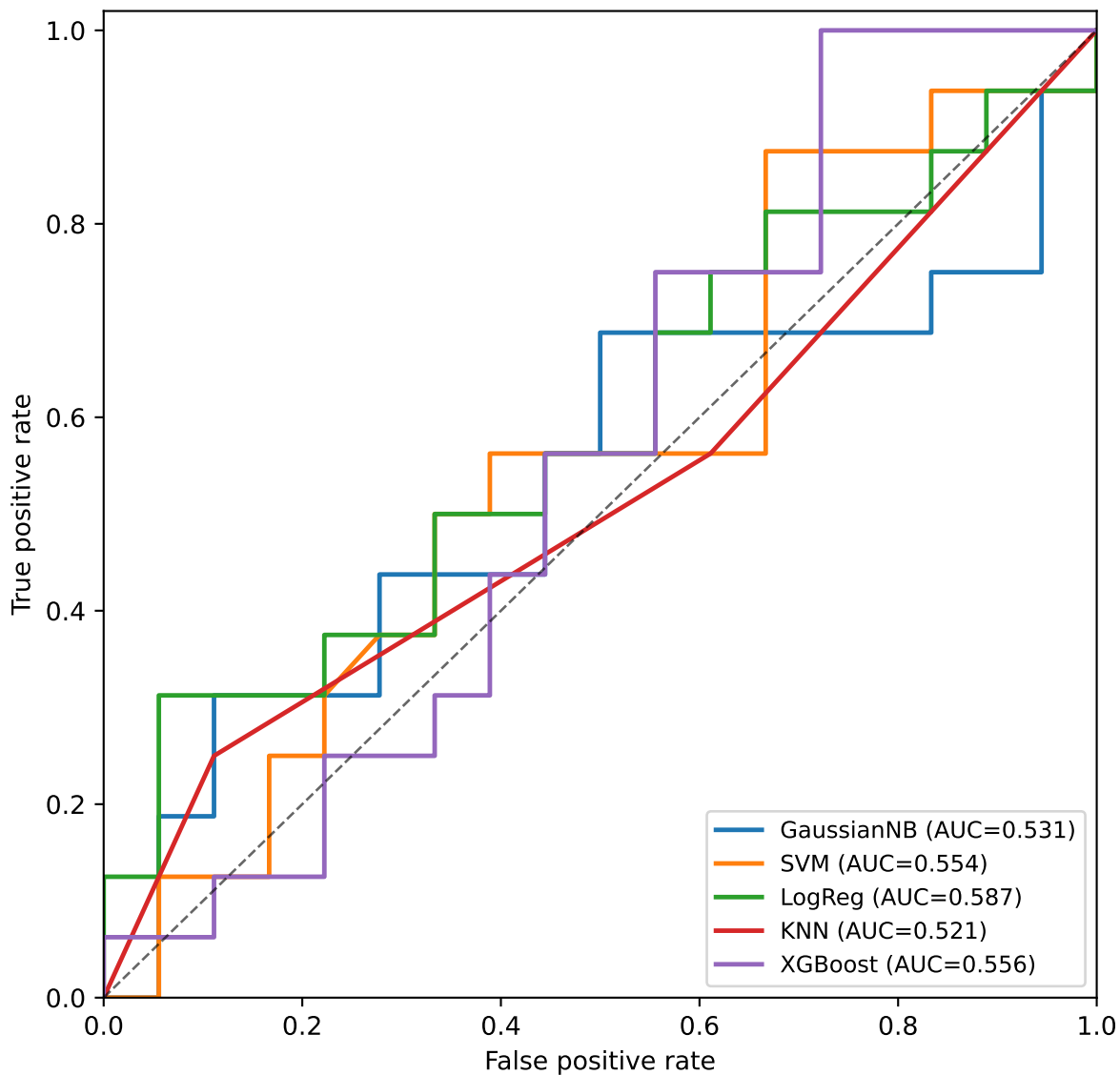
no-GSR: ROC curves (held-out test set)
