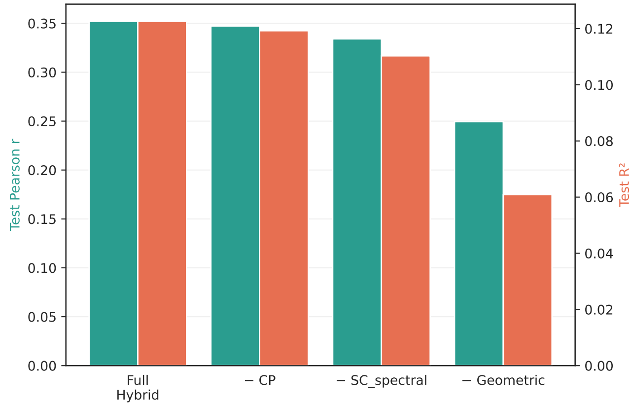
A. Hybrid model with each component removed
