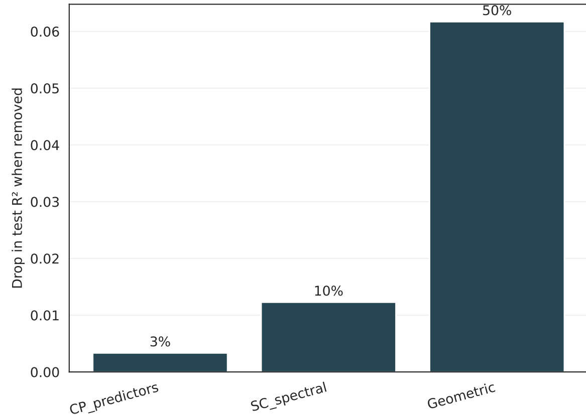
B. Unique contribution of each component (full Hybrid R^2 = 0.123 )
