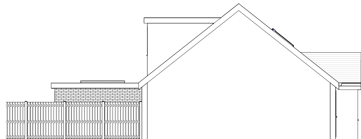
11 Proposed Left Side Elevation 1 : 100
