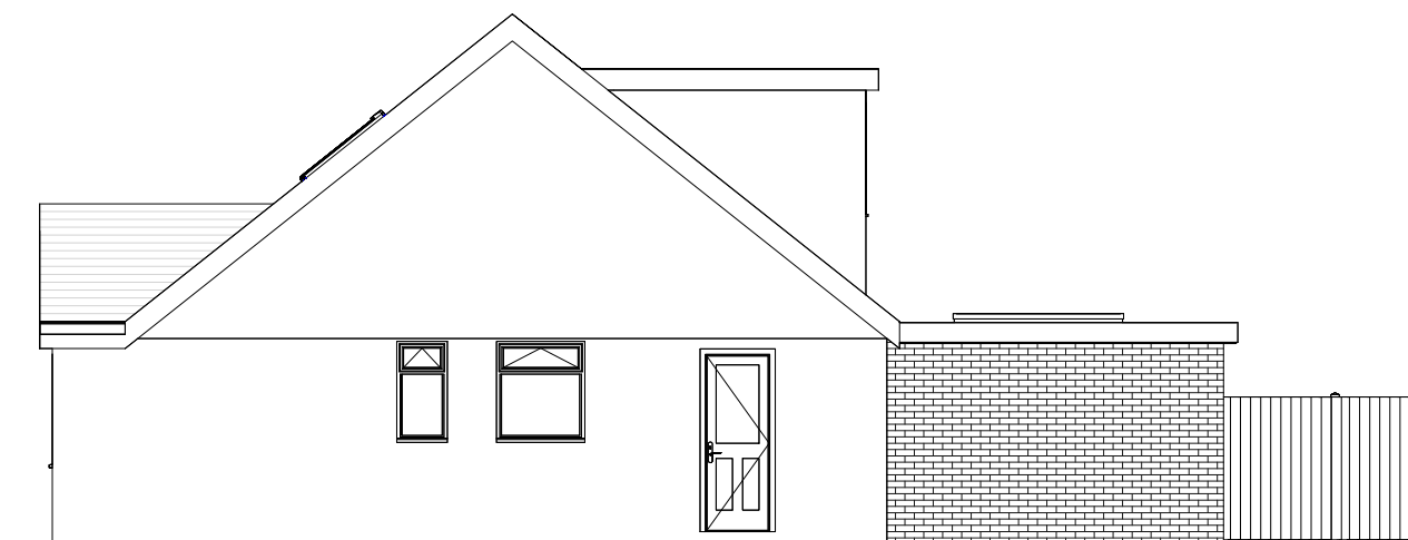
13 Proposed Right Side Elevation 1 : 100
