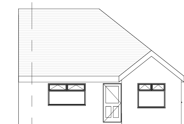
6 Existing Front Elevation 1 : 100
