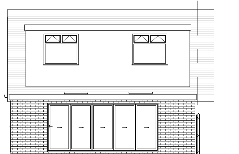
12 Proposed Rear Elevation 1 : 100
