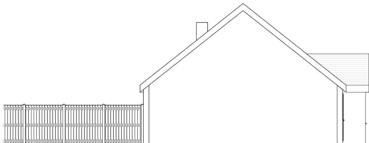
7 Existing Left Side Elevation 1 : 100
