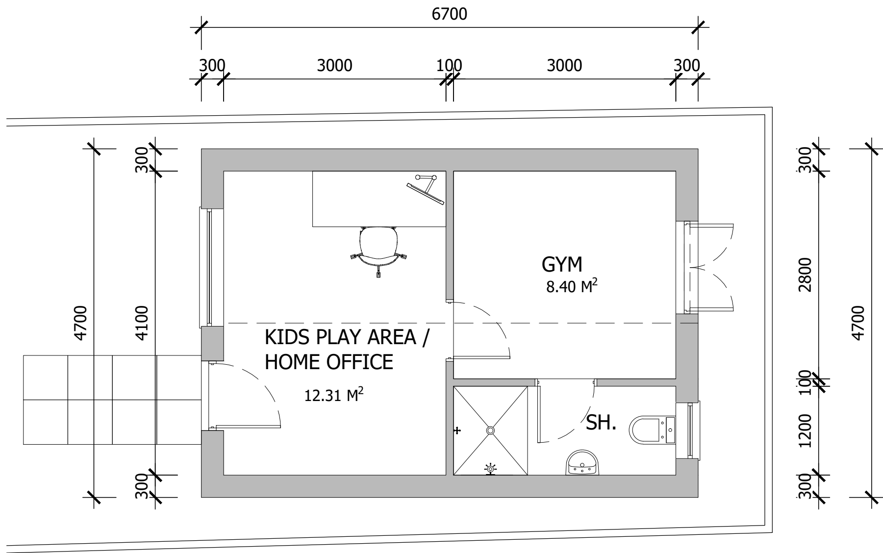
PROPOSED GROUND FLOOR PLAN TOTAL AREA OF OUTBUILDING = 31.49 M² MAIN HOUSE FOOTPRINT AREA = 56.60 M²
