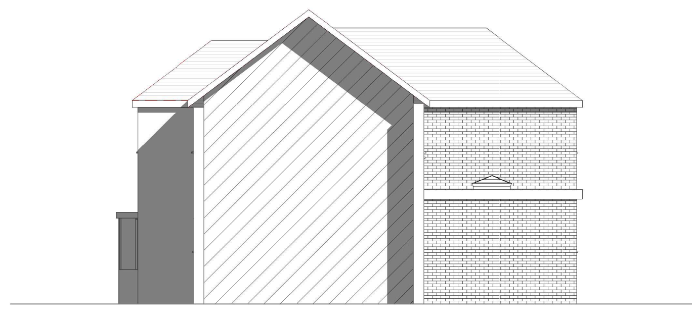
7 Proposed Right Side Elevation 1 : 100
