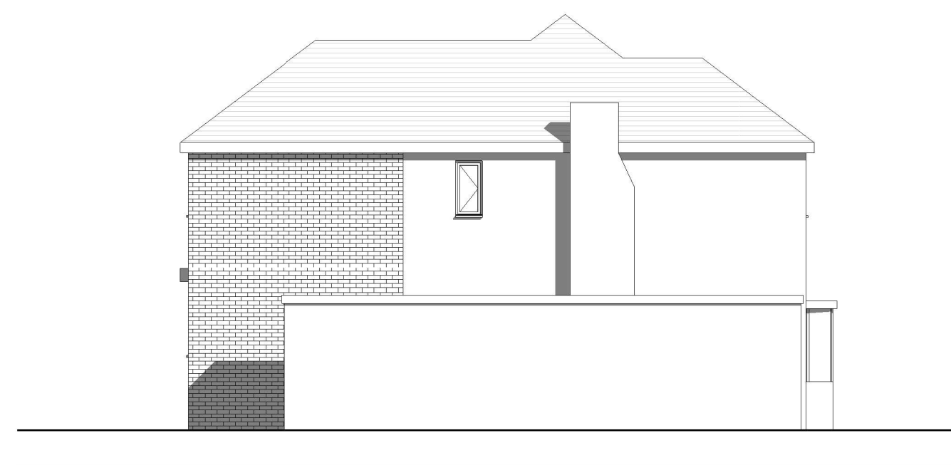
5 Proposed Left Side Elevation 1 : 100
