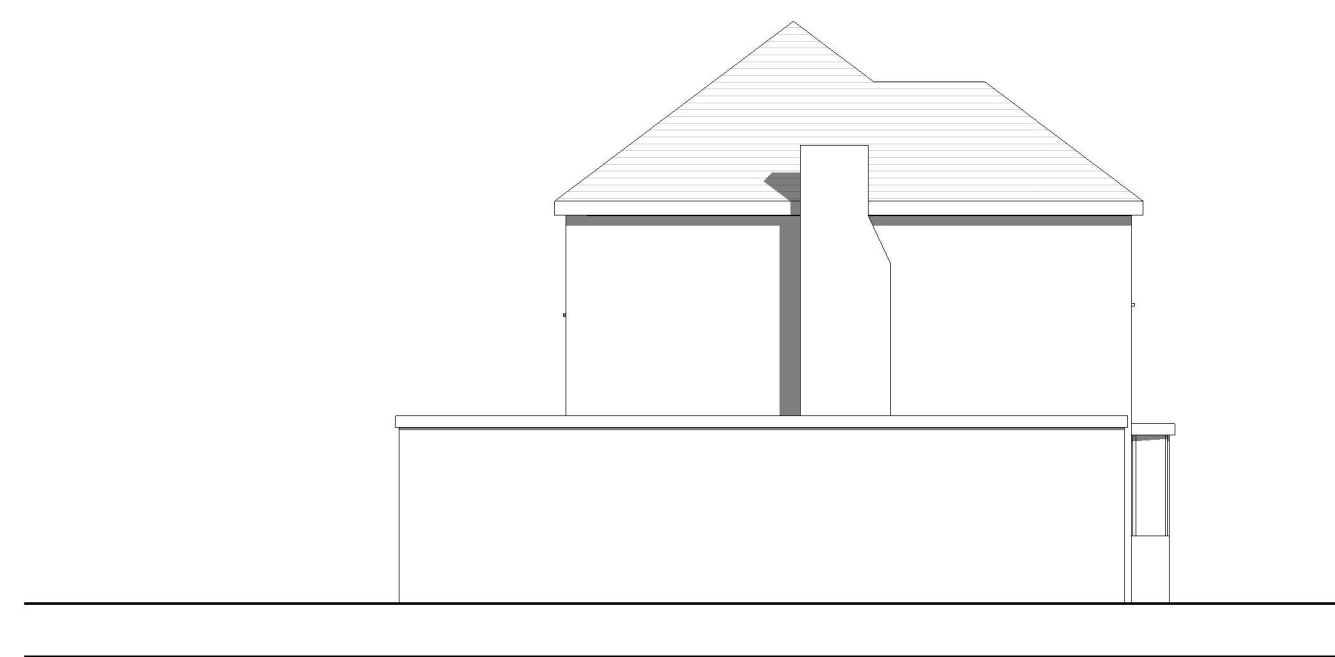
2 Existing Left Side Elevation 1 : 100
