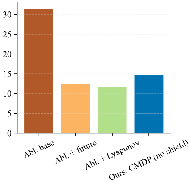
Mean rebuffer (%)
