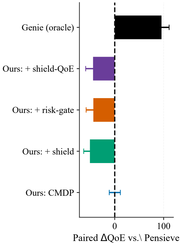
vs.\ Pensieve
