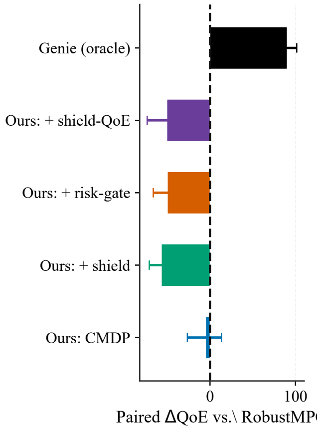
vs.\ RobustMPC
