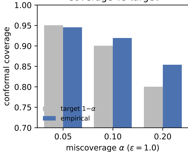
Coverage vs target
