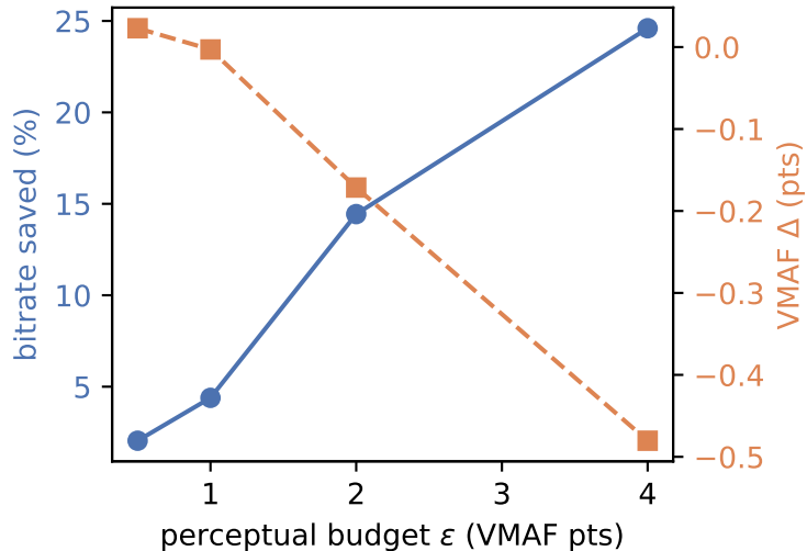
Budget \varepsilon sensitivity ( \alpha = 0.10 )
