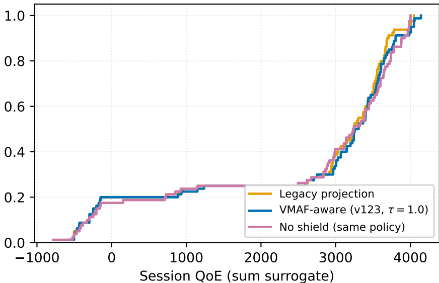
Empirical CDF
