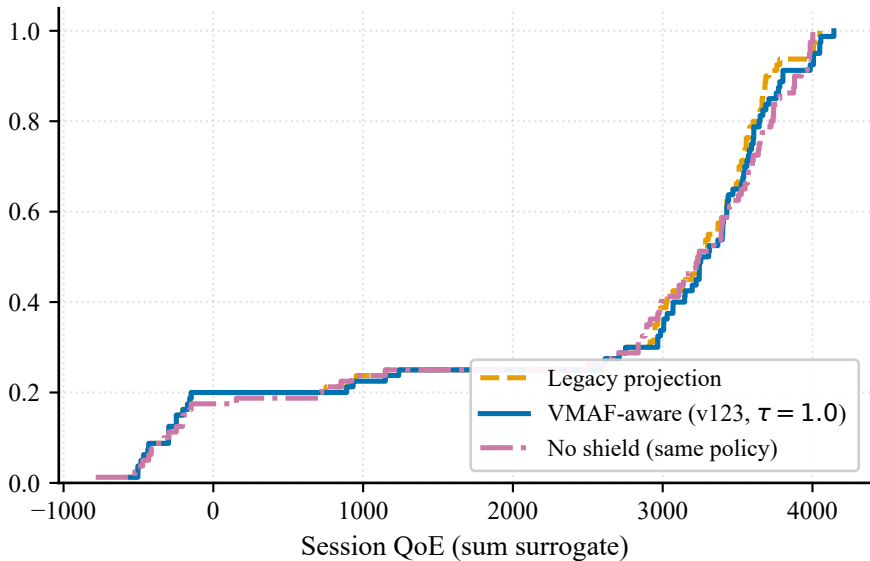
Empirical CDF
