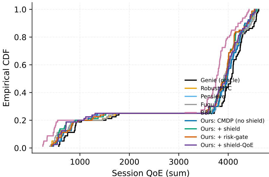
CDF of Episode QoE
