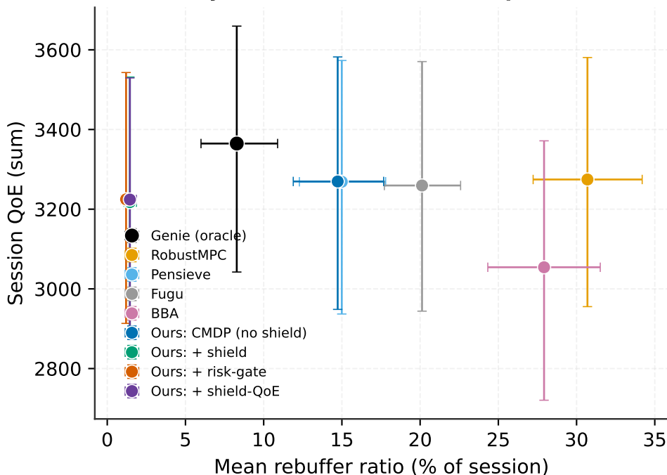
Safety-QoE trade-off (bootstrap 95% CI)
