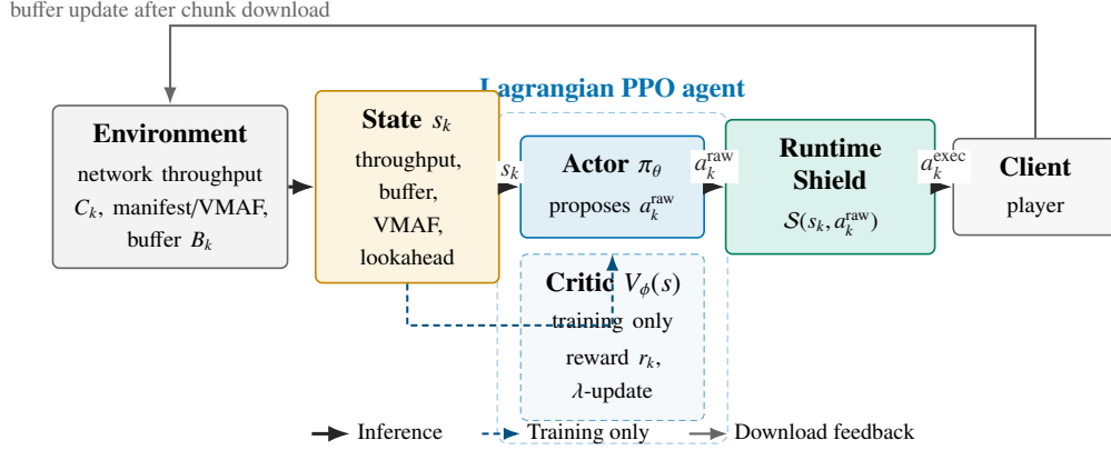
Figure 1: End-to-end control loop. Solid black arrows mark the deployed inference path \text{Environment} \rightarrow \text{State } s_k \rightarrow \text{Actor } \pi_\theta \rightarrow \text{Shield } \mathcal{S}(s_k, a_k^{\text{raw}}) \rightarrow \text{Client} , where the shield’s notation reflects that it consumes both the state and the raw proposal before releasing a_k^{\text{exec}} . The gray arc returns the post-download buffer state to the environment for the next decision step. Dashed blue arrows mark training-only signals feeding the Critic V_\phi(s) (reward r_k and the Lagrangian cues \phi, \psi^{\text{Lya}} that update \lambda_r, \lambda_s ).
