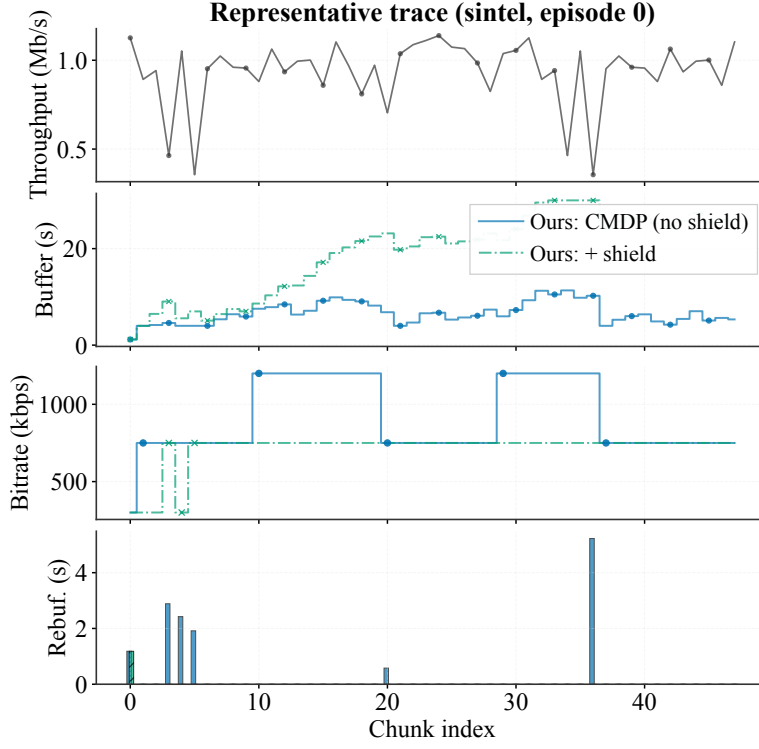
Figure 11: Per-chunk buffer and bitrate trajectories for an example broadband episode. The shielded trajectory (green) avoids buffer depletion during the displayed throughput reductions.
