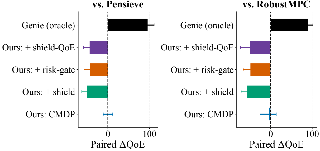
Figure 4: Paired QoE differences relative to Pensieve (left) and RobustMPC (right), with 95% bootstrap confidence intervals within each video and pooled across videos.
