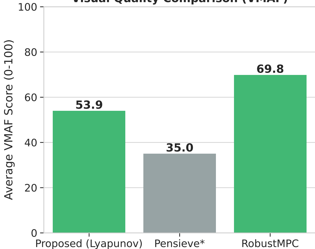
Visual Quality Comparison (VMAF)
