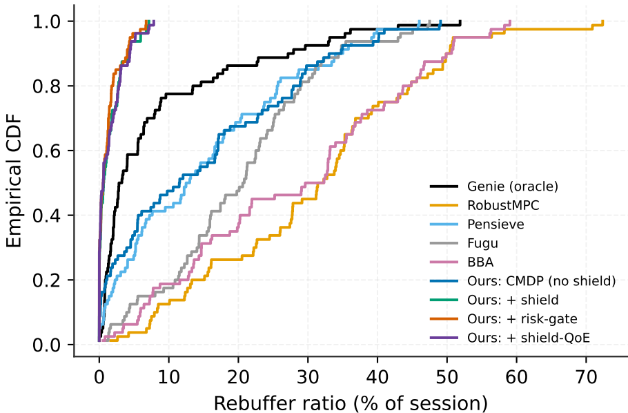
CDF of Episode rebuffer %
