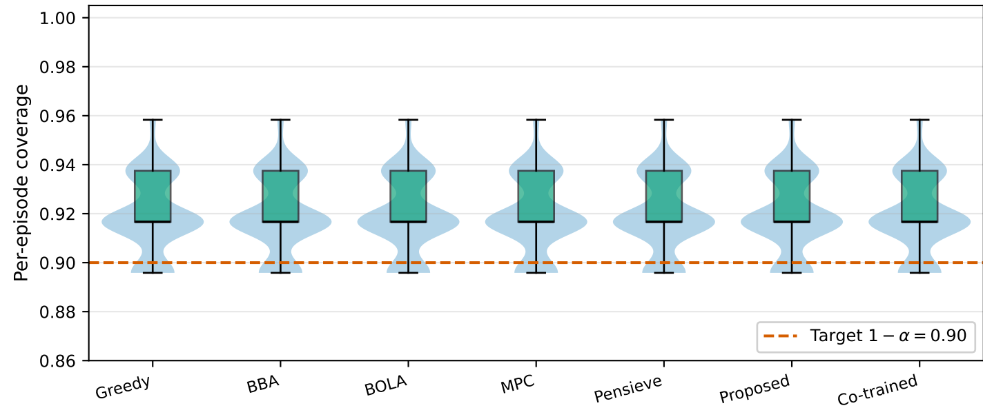
Conformal coverage per episode (certified arm, \alpha = 0.10 )
