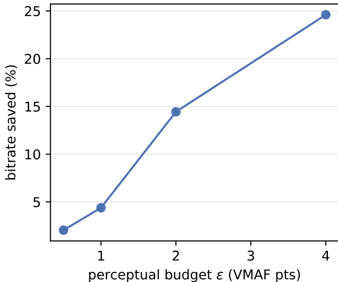
Budget \varepsilon sensitivity ( \alpha = 0.10 )
