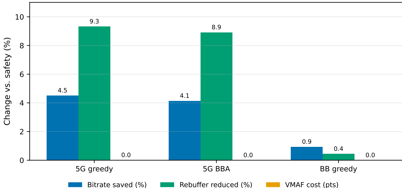
CPS banking: magnitude, perceptual cost, and regime ( \epsilon = 1.0 )
