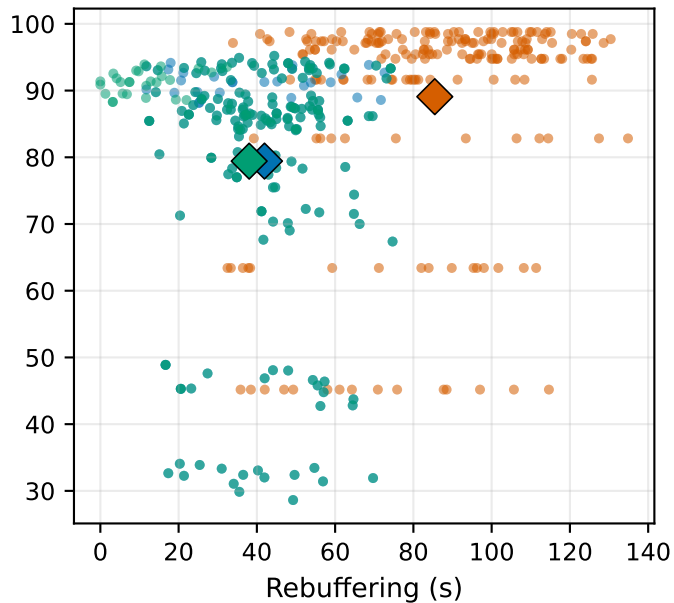
Mean VMAF
