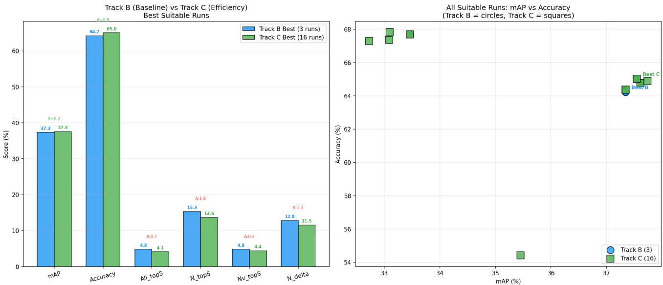
Figure 7 - Track B vs Track C Comparison
