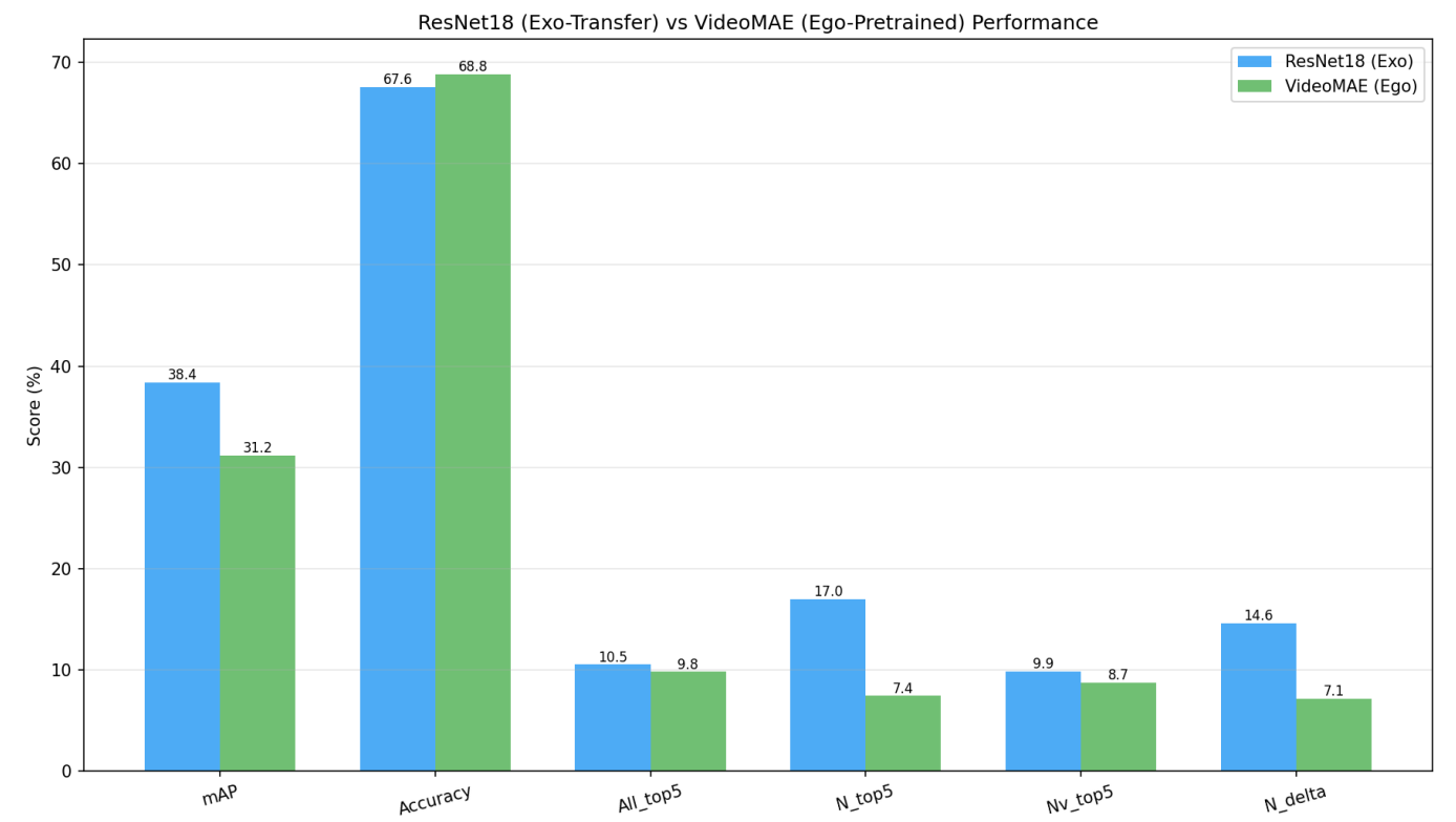
Figure 6 - Backbone Metrics Comparison
