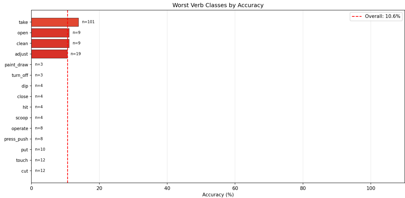
Figure 17 - Worst Verb Classes
