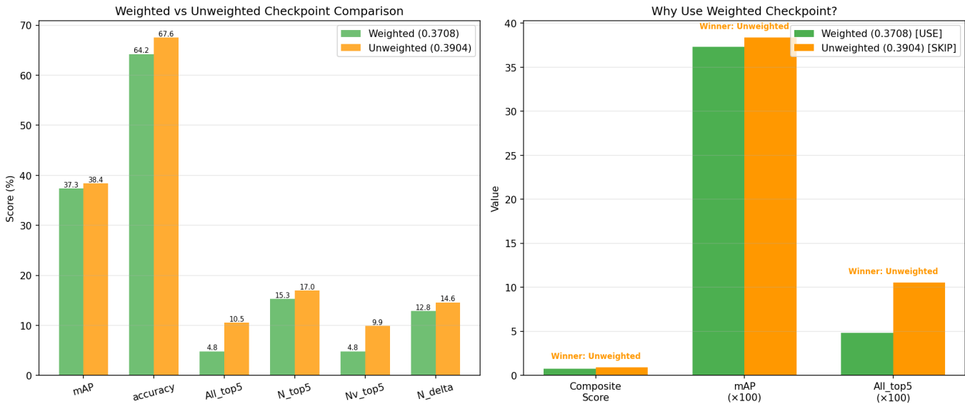
Figure 1 - Weighted vs Unweighted Comparison
