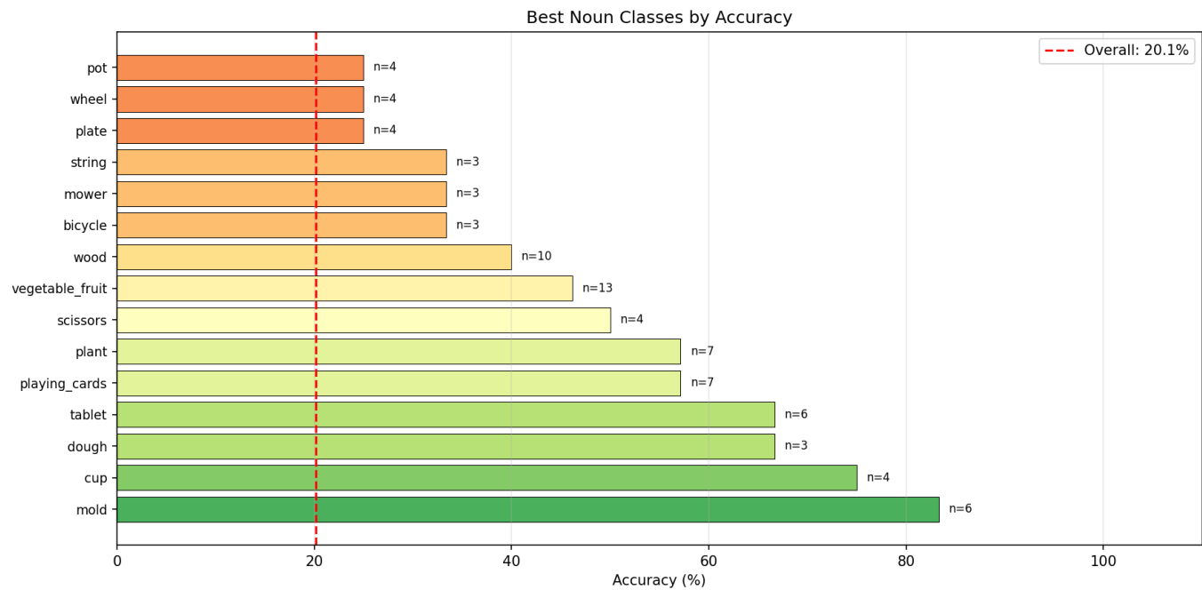
Figure 16 - Best Noun Classes
