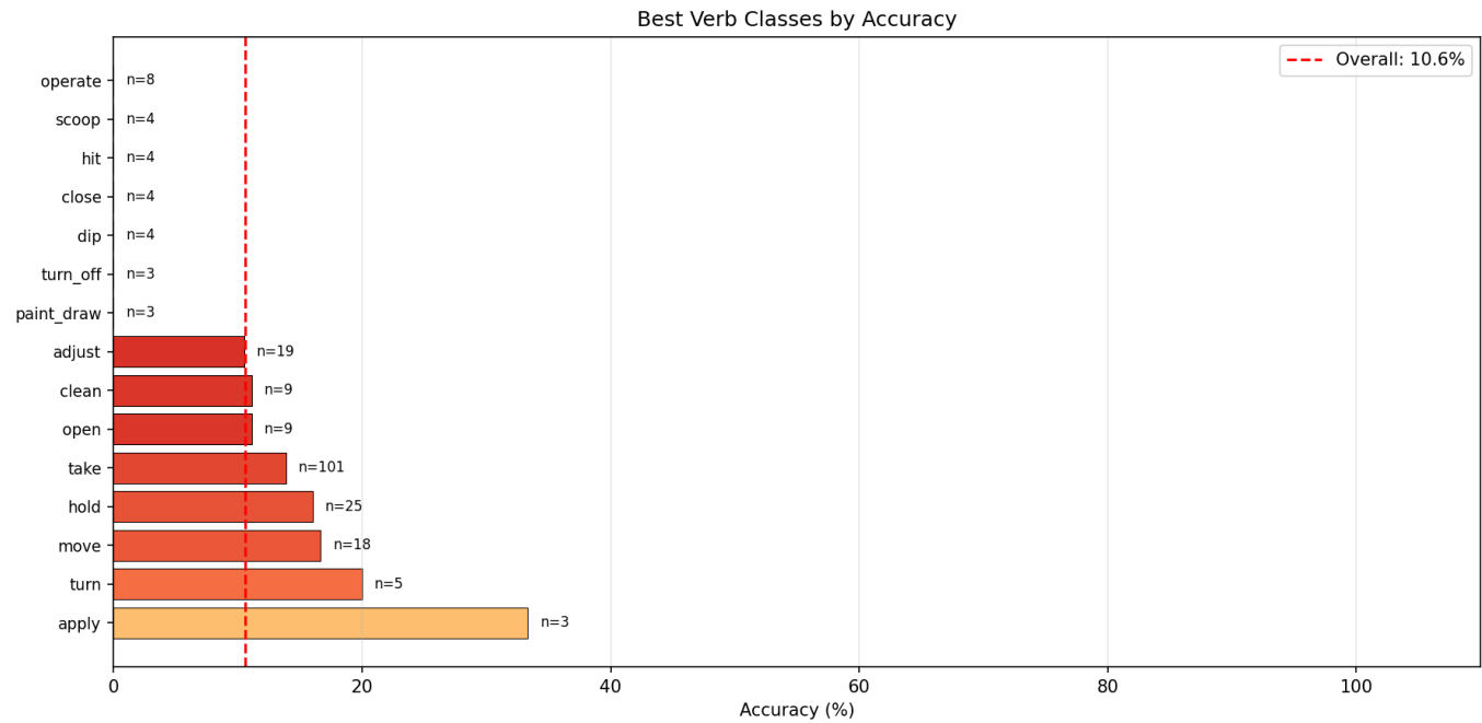
Figure 18 - Best Verb Classes
