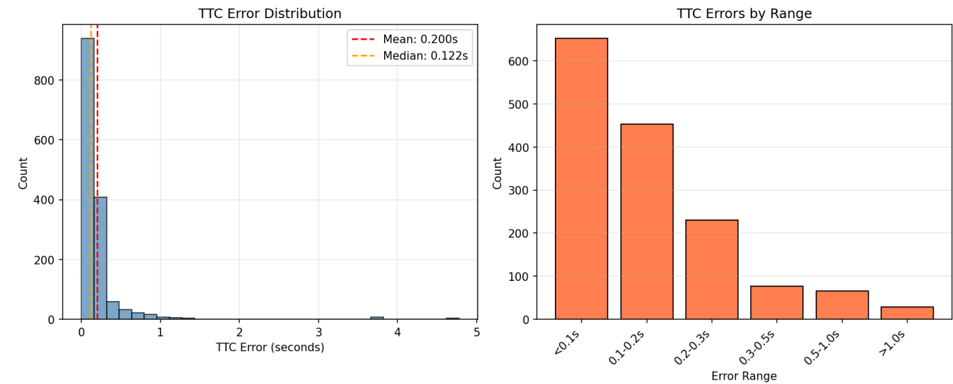
Figure 20 - TTC Error Distribution
