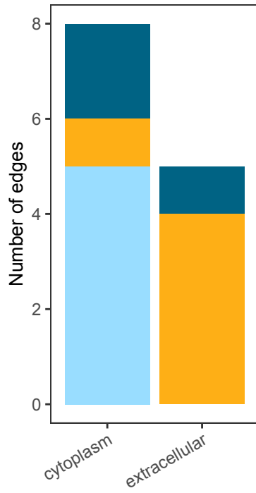
KRAS down
