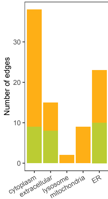
KRAS up
