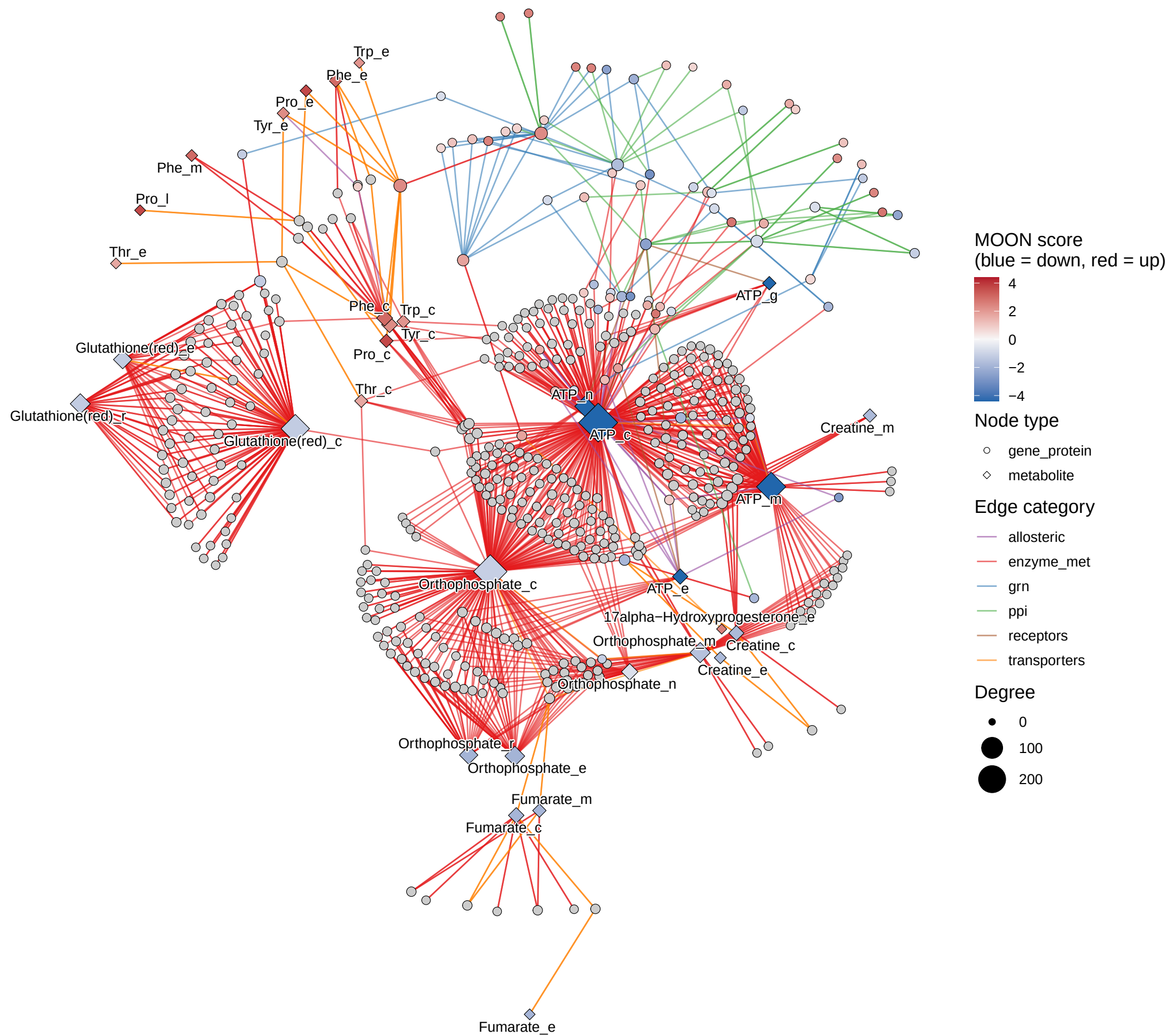
Case study 2, WT_6h -- GEM-instance-merged network
