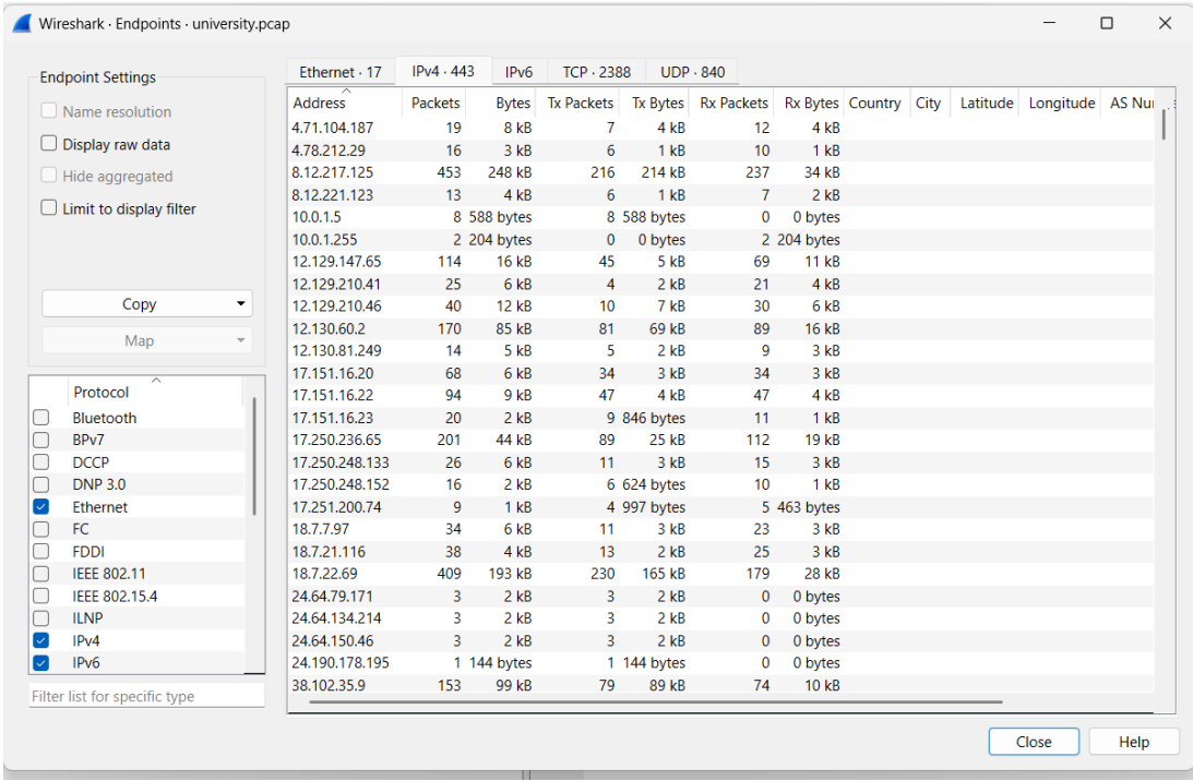
FIGURE 1.1 – Endpoints IPv4
