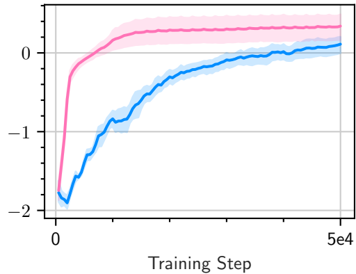
CylinderJet2D-medium-v0
