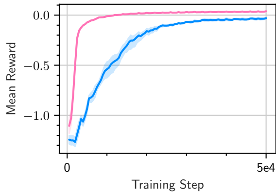
CylinderRot2D-easy-v0
