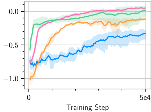
CylinderJet3D-medium-v0
