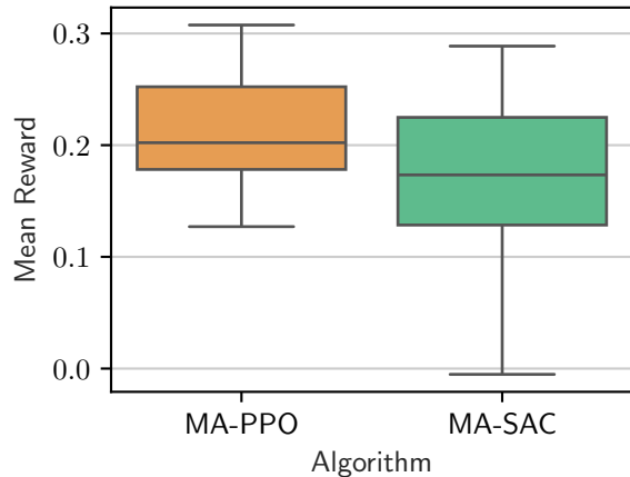
TCFSmall3D-both-easy-v0
