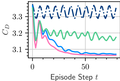
Drag Coefficient
