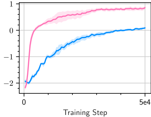
CylinderRot2D-hard-v0
