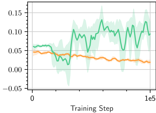
TCFLLarge3D-both-medium-v0
