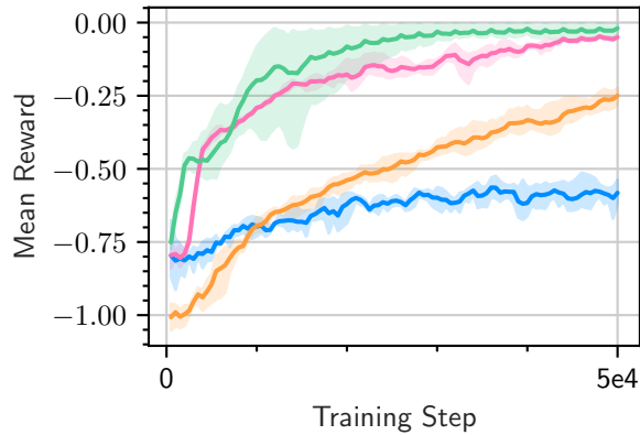
CylinderJet3D-easy-v0
