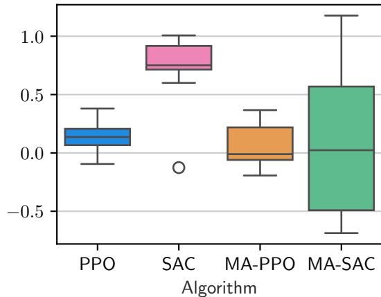
RBC2D-medium-v0
