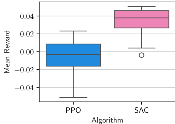
CylinderRot2D-easy-v0
