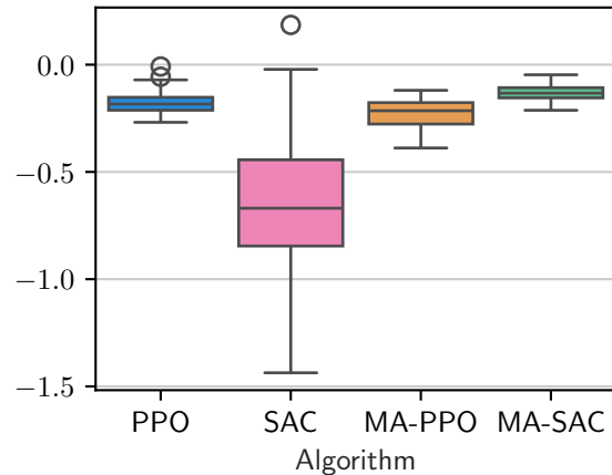
CylinderJet3D-hard-v0
