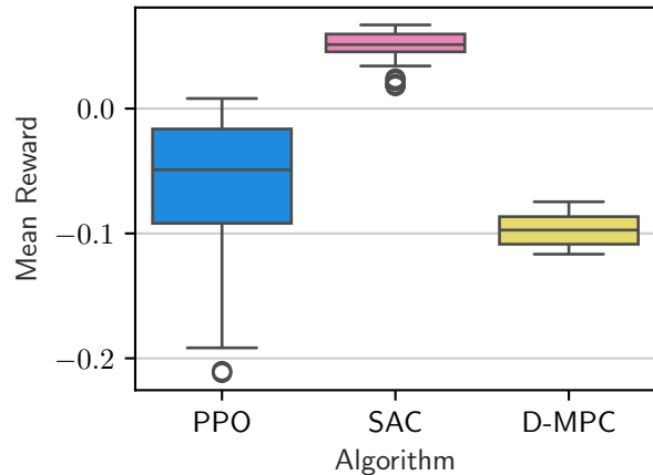
CylinderJet2D-easy-v0
