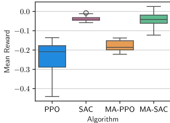
CylinderJet3D-easy-v0
