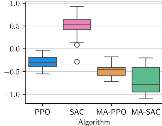
RBC2D-hard-v0
