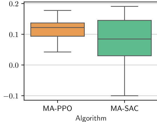
TCFSmall3D-both-hard-v0
