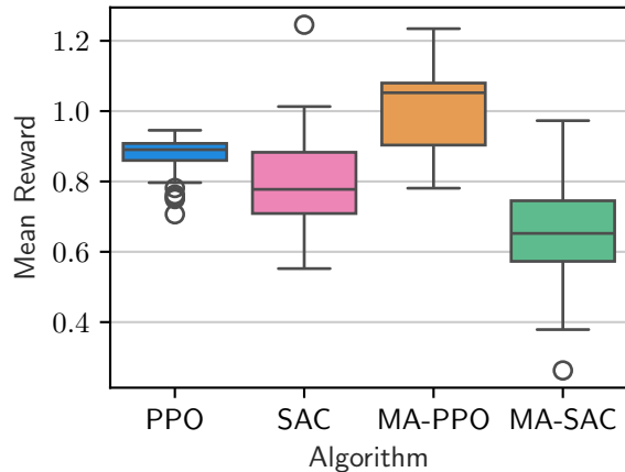
RBC2D-easy-v0
