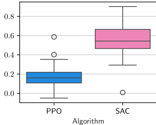
CylinderRot2D-hard-v0
