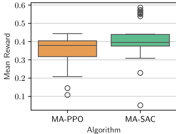
RBC3D-easy-v0
