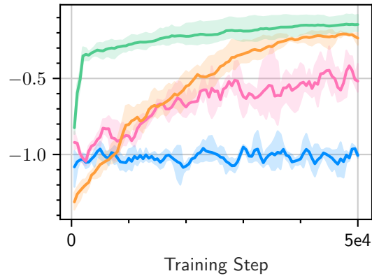
CylinderJet3D-hard-v0
