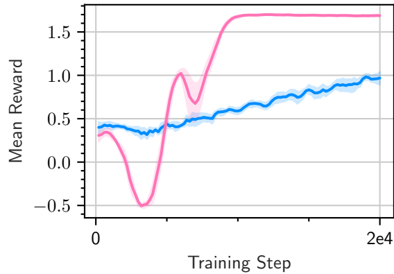
Airfoil2D-easy-v0
