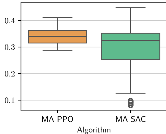
RBC3D-hard-v0
