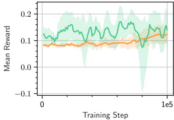
TCFLLarge3D-both-easy-v0
