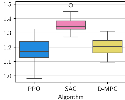
CylinderJet2D-hard-v0
