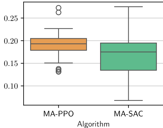
TCFSmall3D-both-medium-v0
