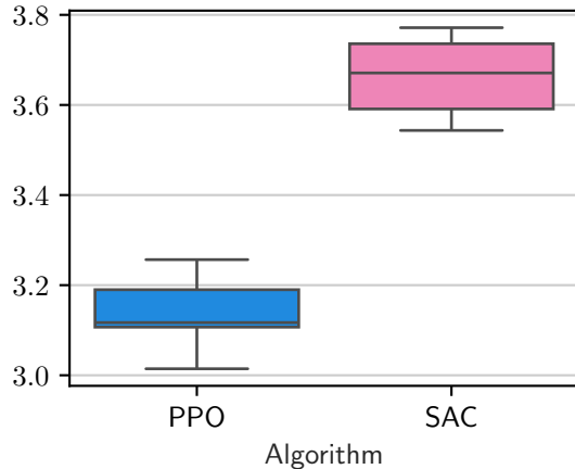
Airfoil2D-medium-v0
