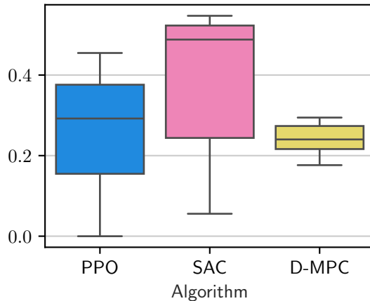
CylinderJet2D-medium-v0
