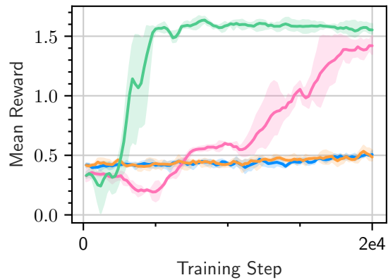
Airfoil3D-easy-v0
