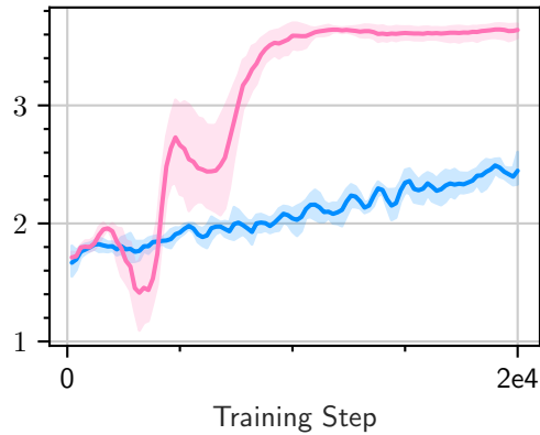
Airfoil2D-medium-v0
