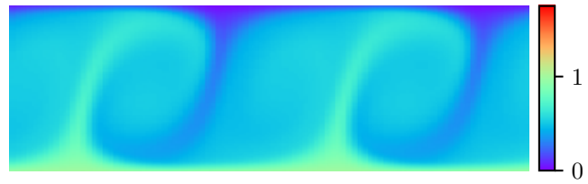
Hard
