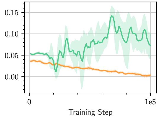
TCFLLarge3D-both-hard-v0
