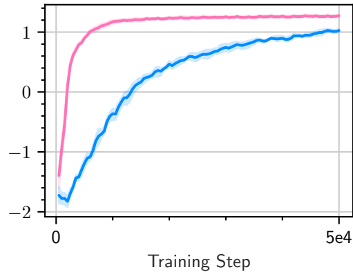
CylinderJet2D-hard-v0
