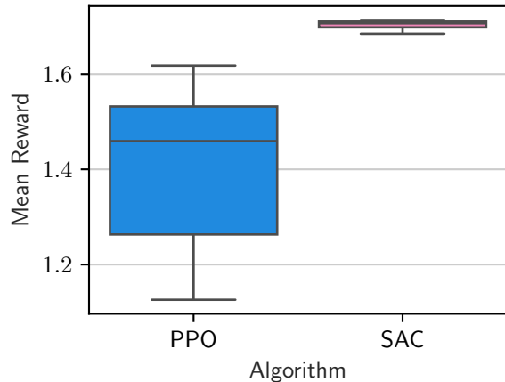
Airfoil2D-easy-v0
