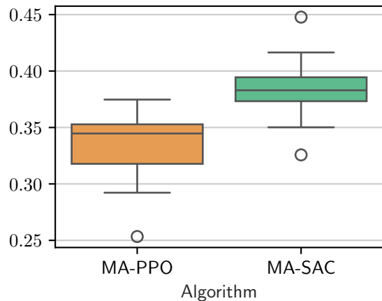
RBC3D-medium-v0
