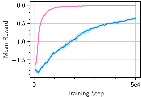
CylinderJet2D-easy-v0
