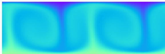
Medium
