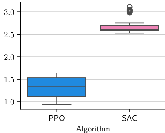
Airfoil2D-hard-v0
