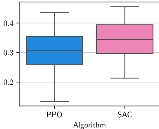
CylinderRot2D-medium-v0
