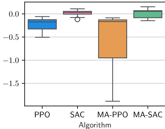
CylinderJet3D-medium-v0
