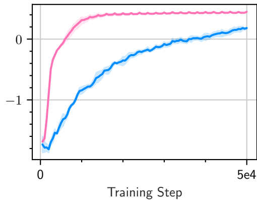
CylinderRot2D-medium-v0
