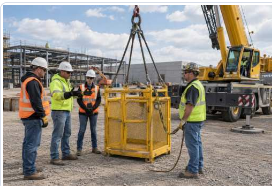
Approved basket - Dedicated rigging - Stabilizers - Trial lift - Communication - Rescue
