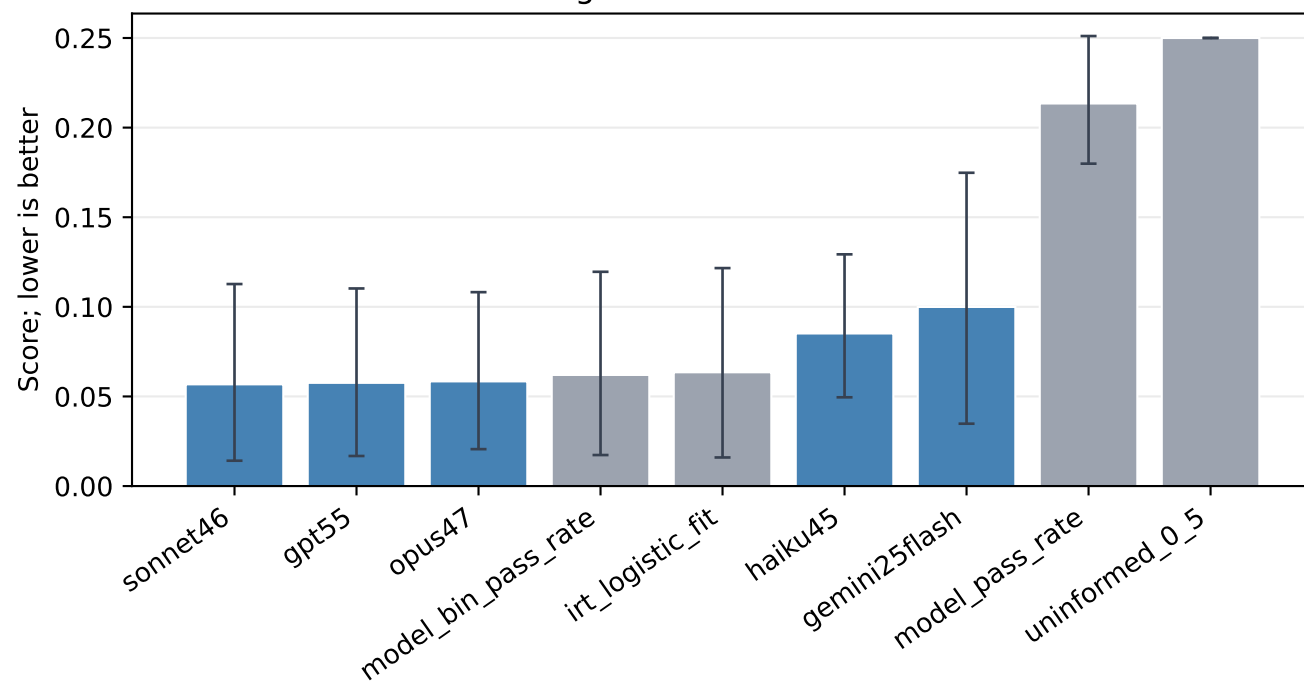
Target Bin 1: Brier Score
