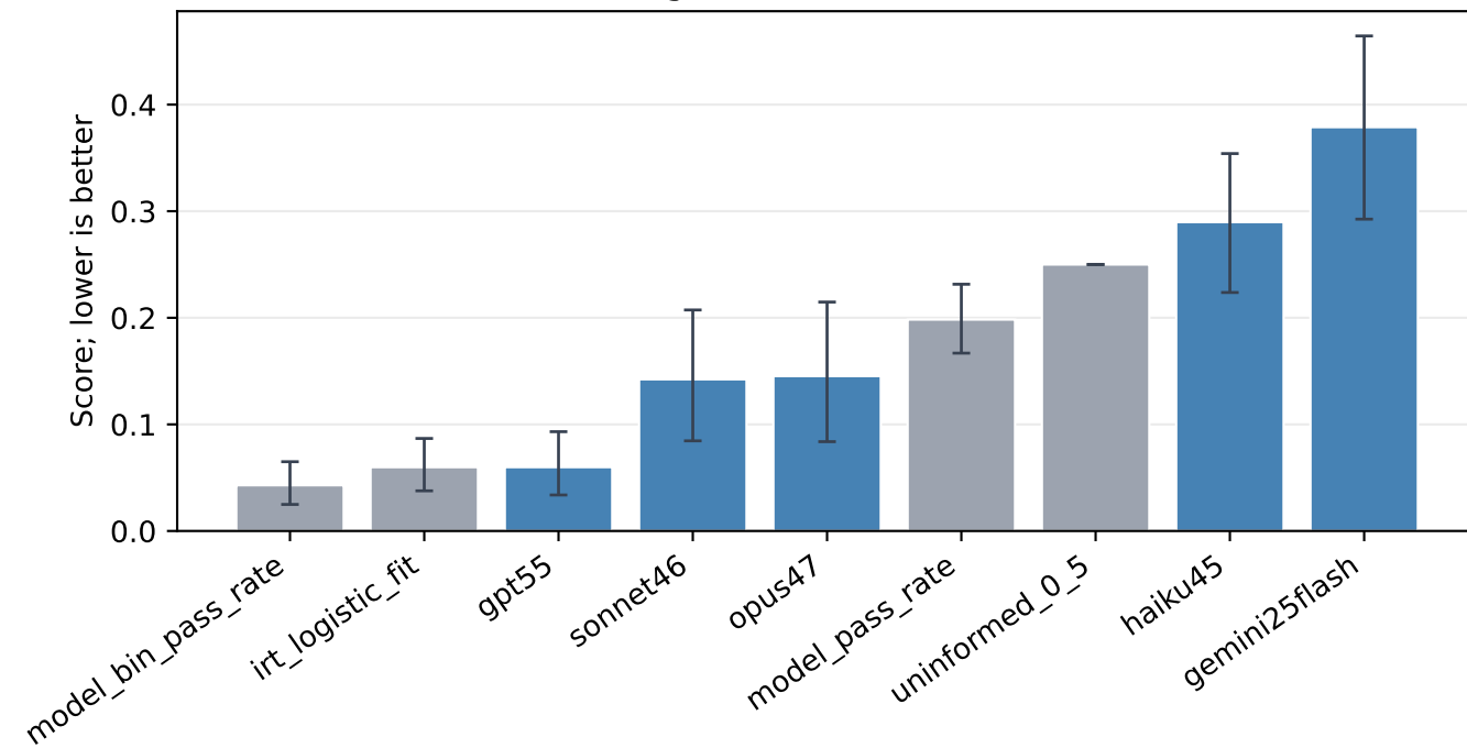
Target Bin 2: Brier Score
