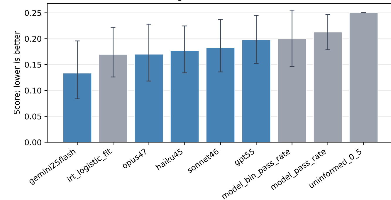
Target Bin 3: Brier Score
