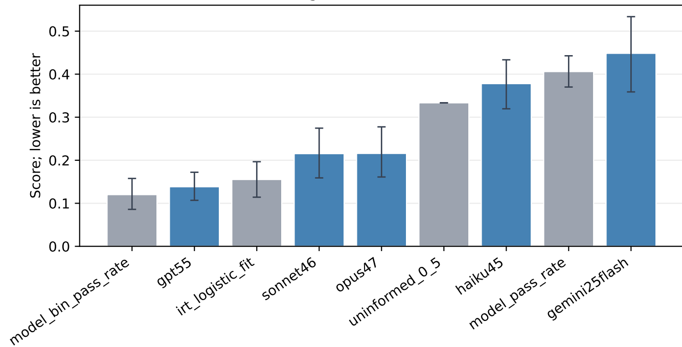
Target Bin 2: Beta CRPS
