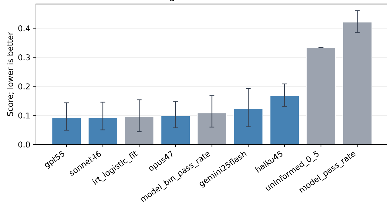
Target Bin 1: Beta CRPS
