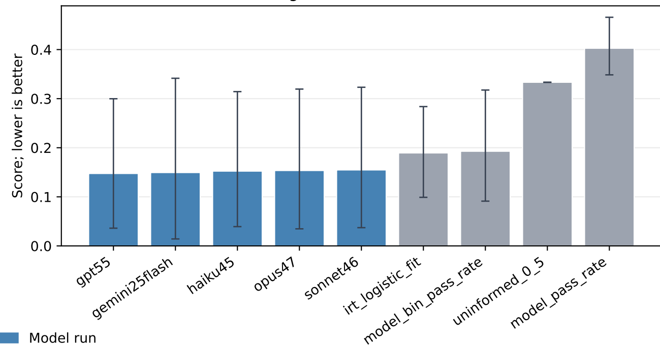
Target Bin 3: Beta CRPS
