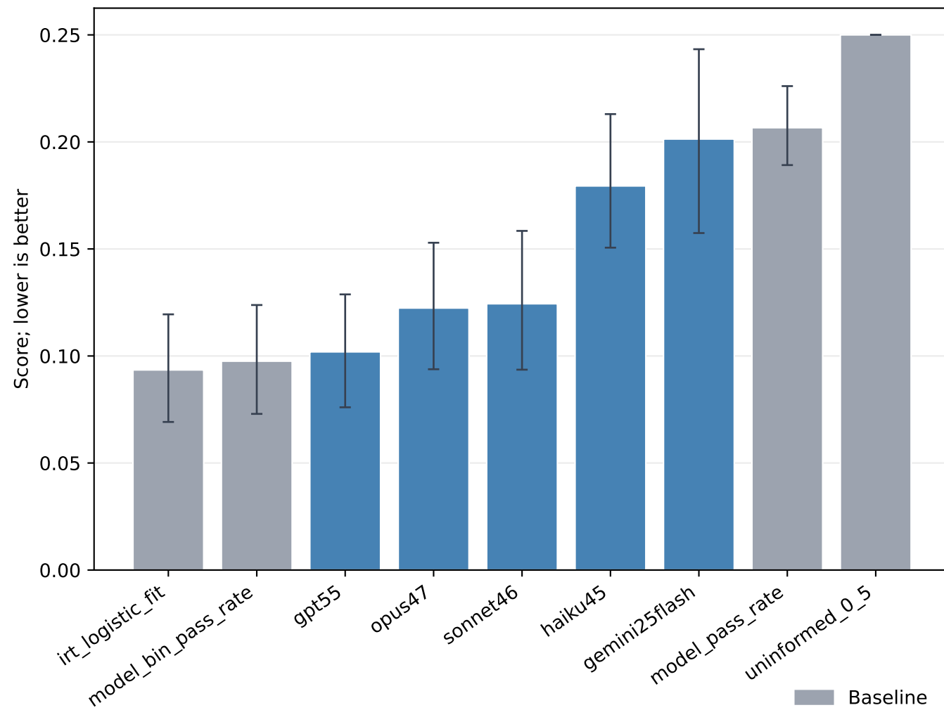
Brier Score
