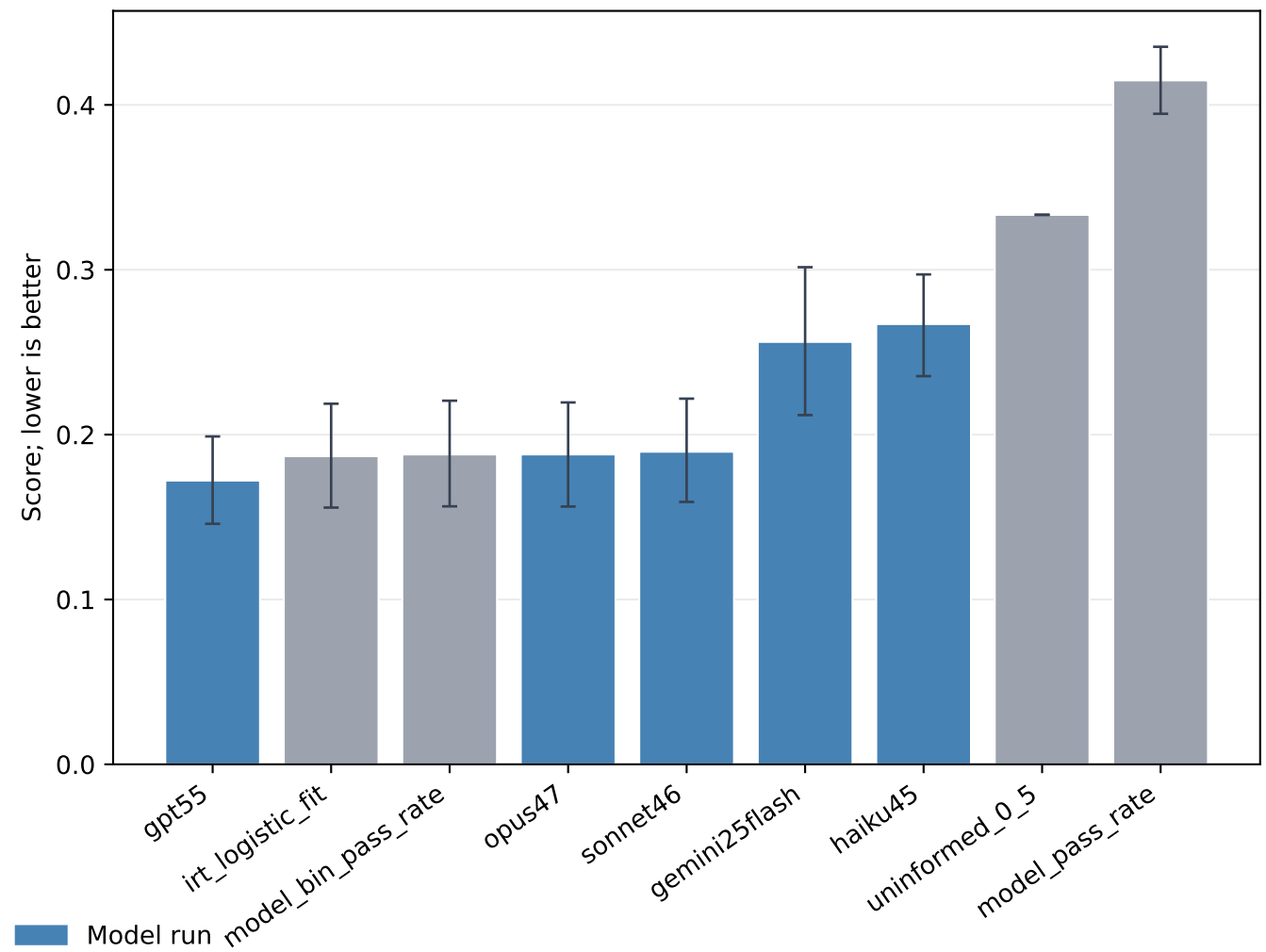
Beta CRPS
