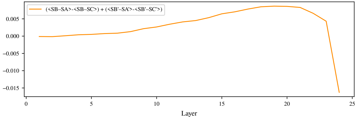
Combined Cosine Similarity Difference for GPT-2-medium
