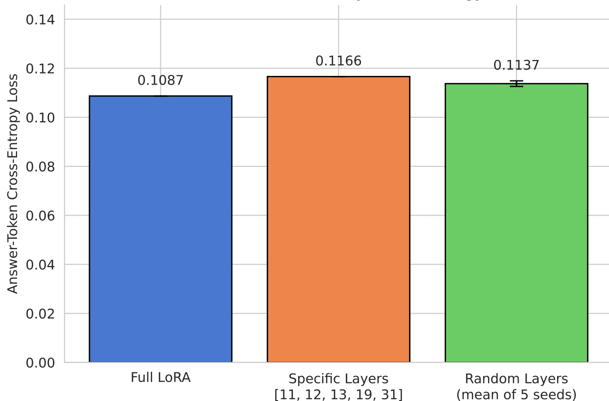
Answer-Token Loss by LoRA Strategy
