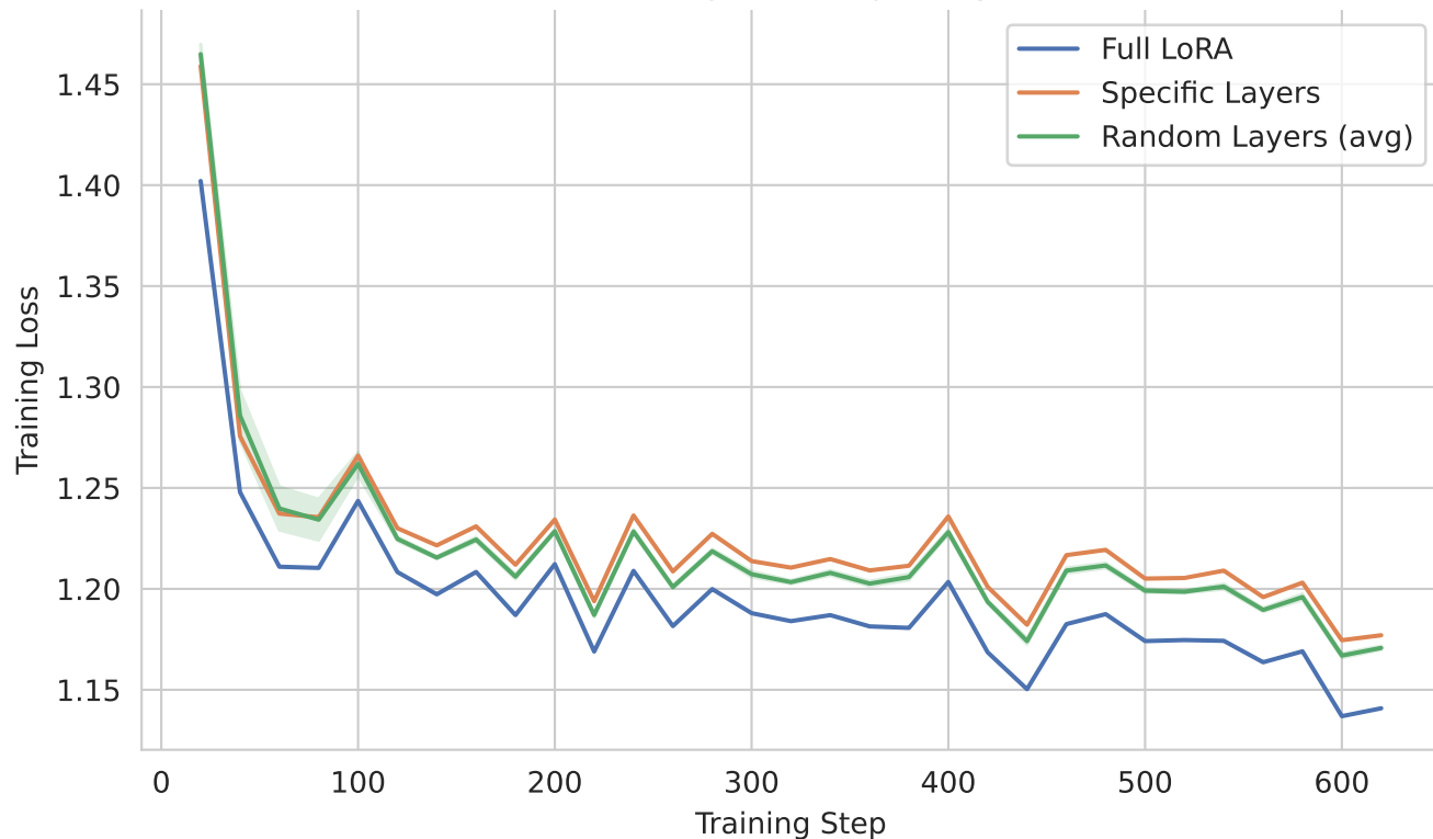
Training Loss Trajectory
