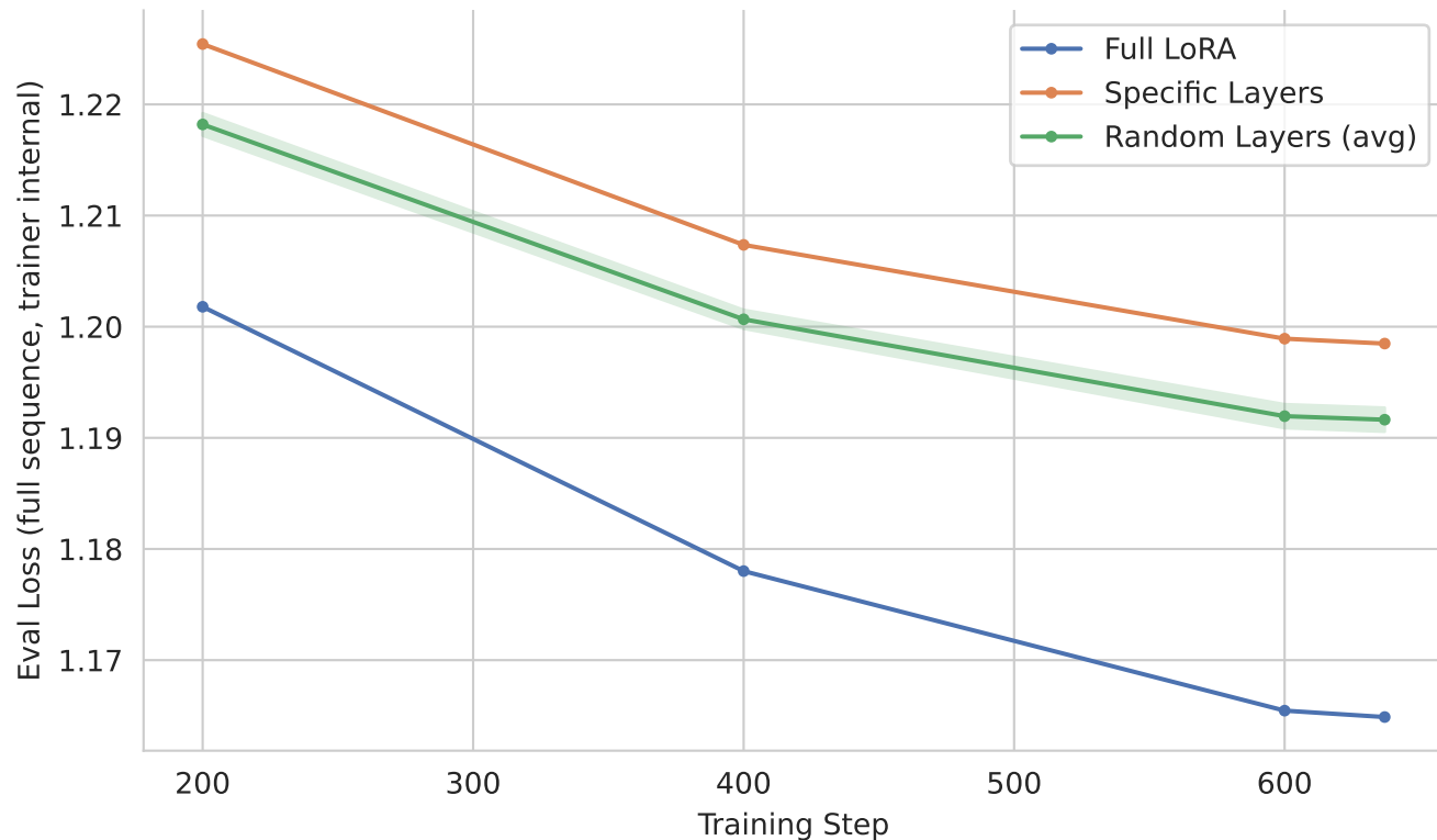
Validation Loss Trajectory (full-seq) (shaded = \pm 1 std across random seeds)
