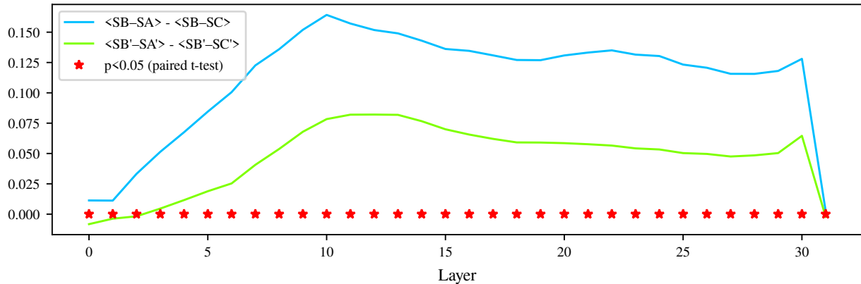
Average Cosine Similarity Difference for Finance-Llama
