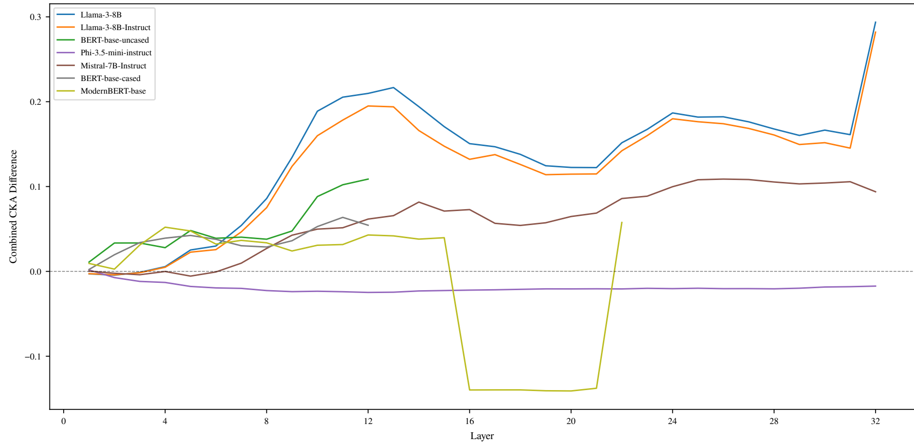
Combined CKA Difference — All Base/General Models
