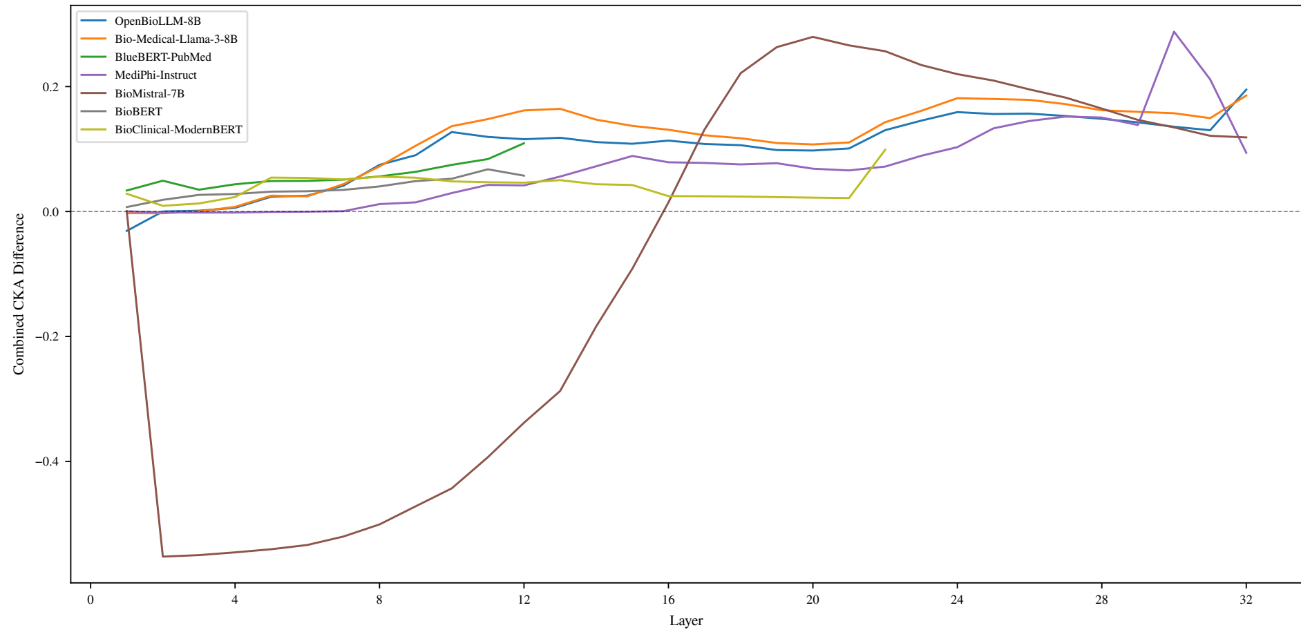
Combined CKA Difference — All Biomedical Models
