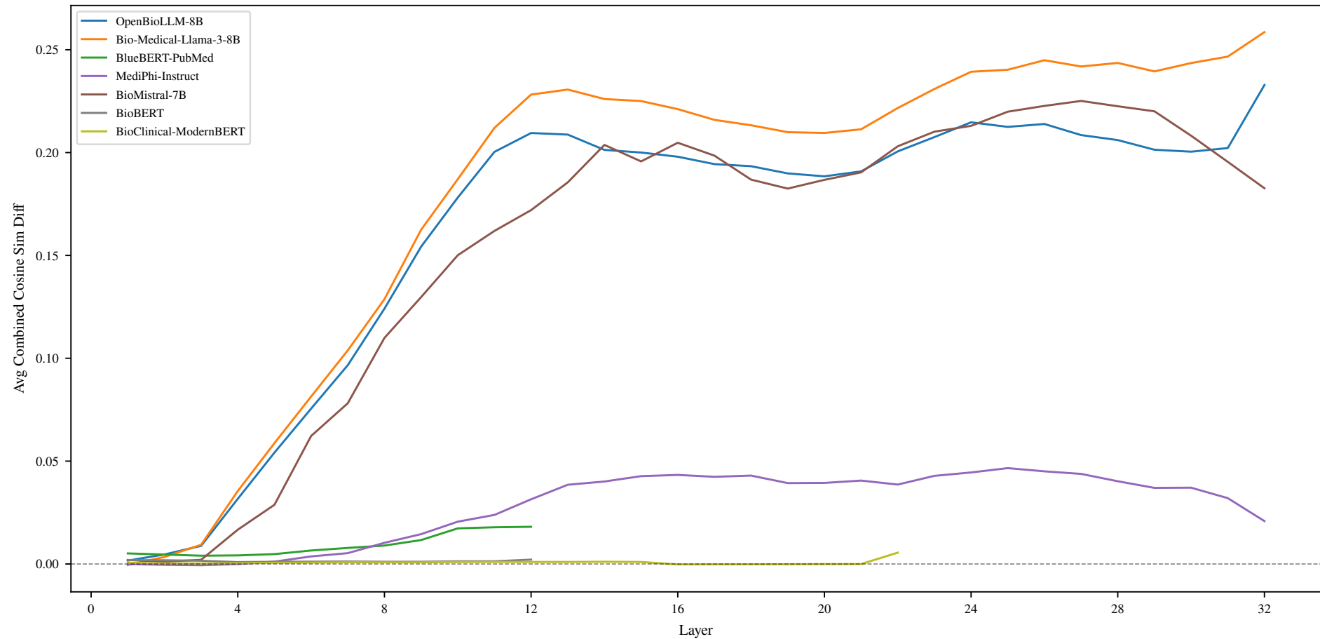
Combined Cosine Similarity Difference — All Biomedical Models
