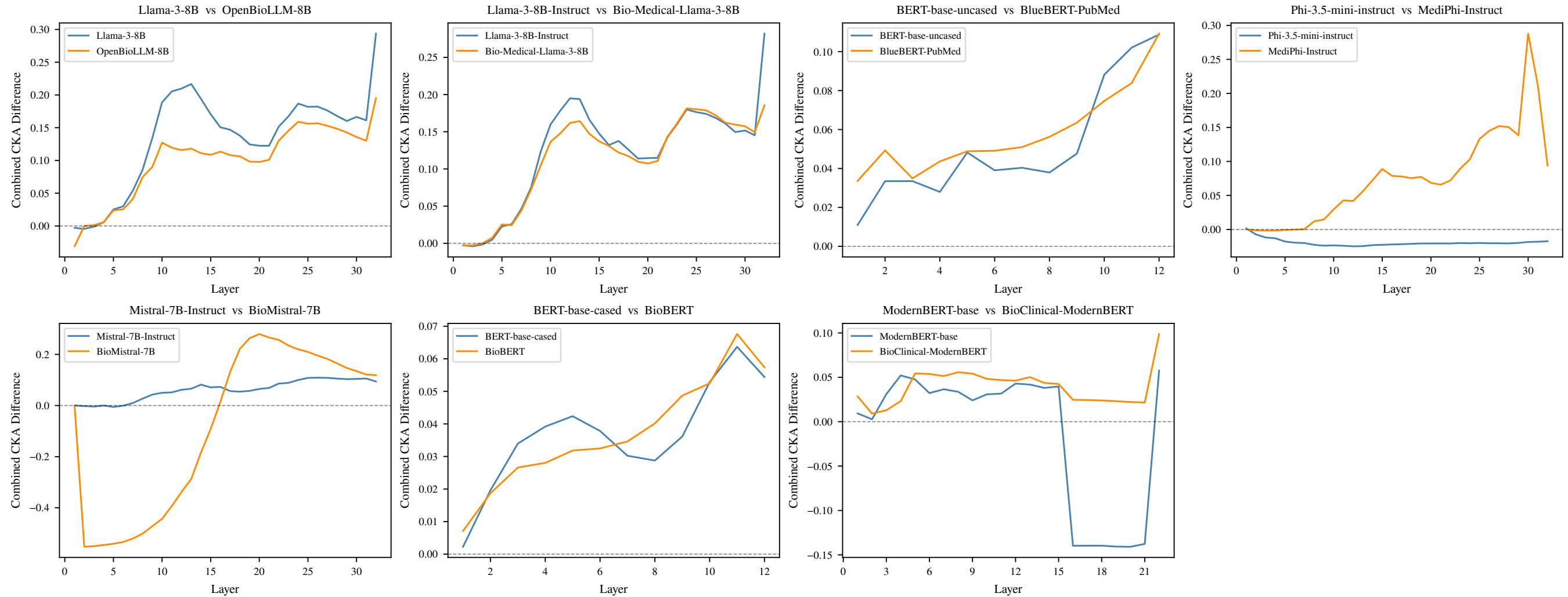
Combined CKA Difference by Layer — General vs Biomedical Models
