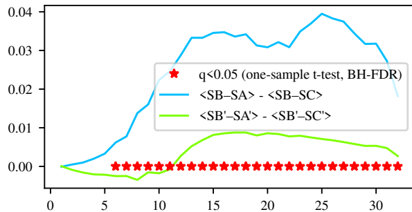
Independent Components
