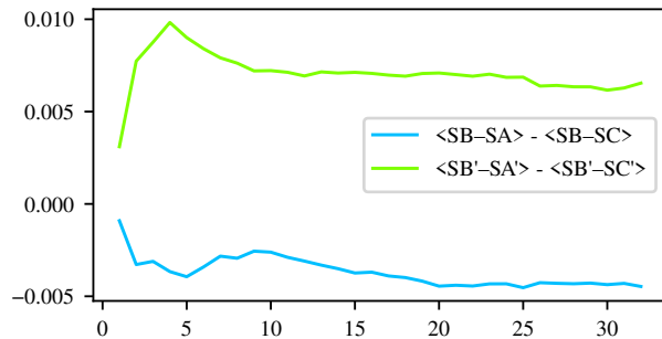
Independent Components
