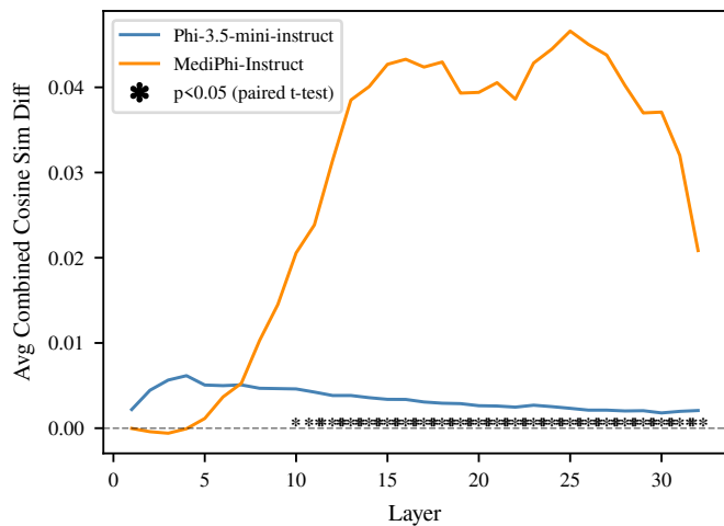
Phi-3.5-mini-instruct vs MediPhi-Instruct
