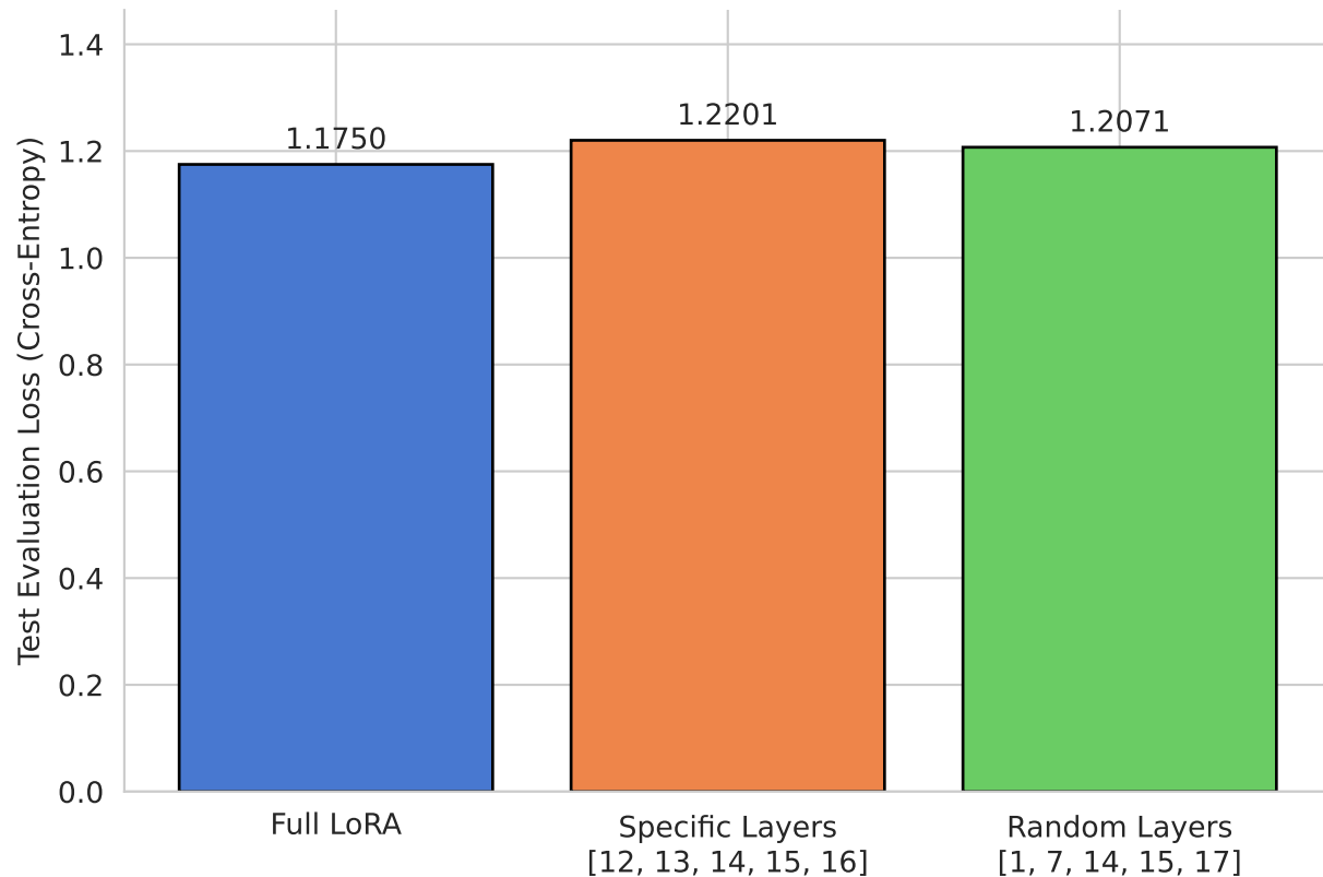
Test-set Loss by LoRA Strategy
