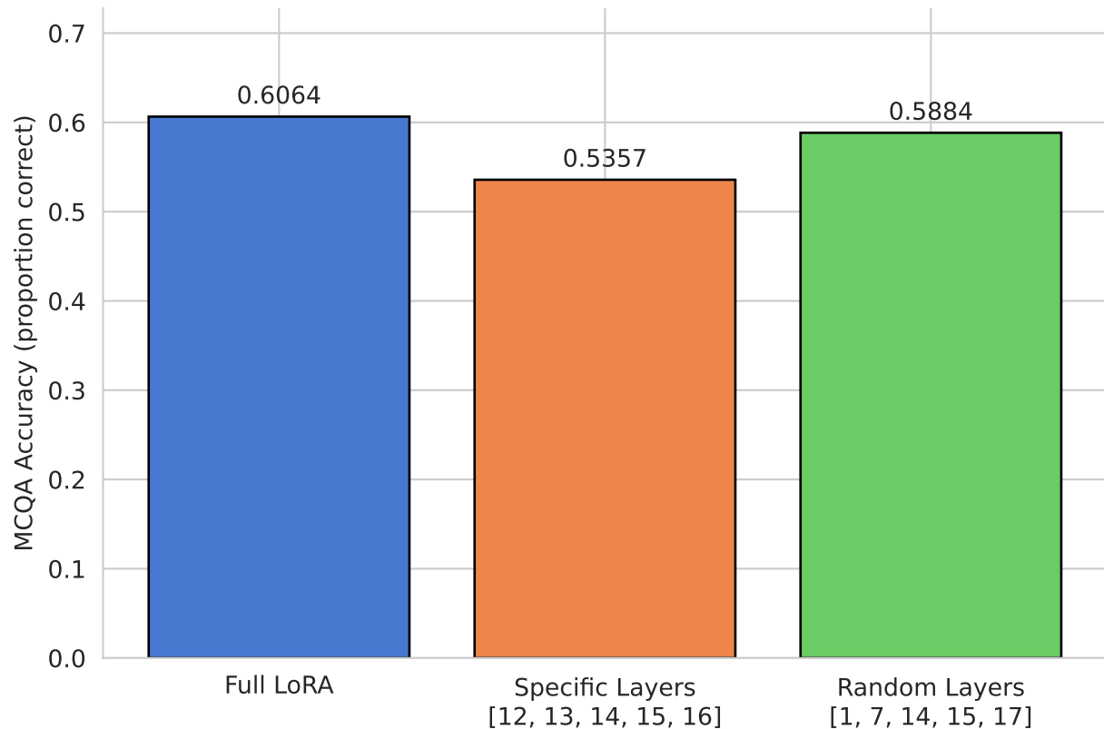
MCQA Answer Accuracy by LoRA Strategy
