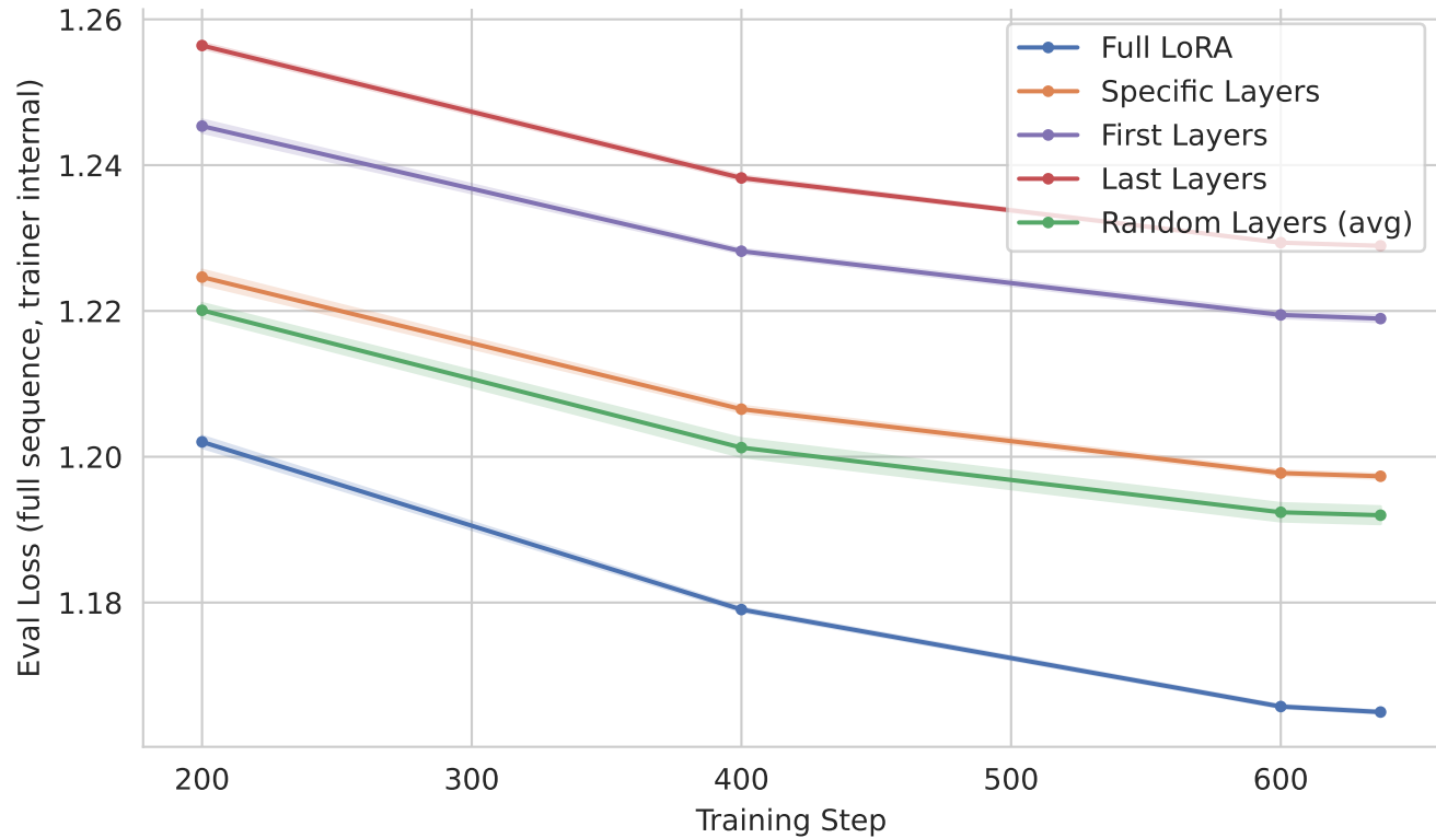
Validation Loss Trajectory (full-seq) (shaded = \pm 1 std across runs)
