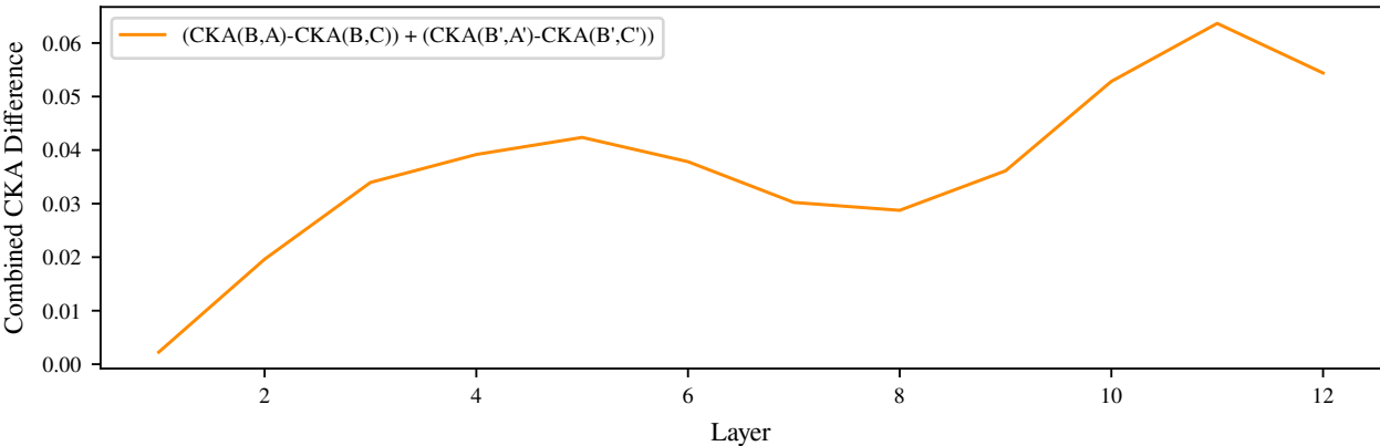
Combined CKA Difference for BERT-base-cased
