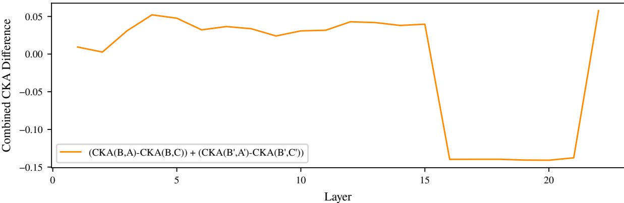
Combined CKA Difference for ModernBERT-base
