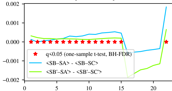
Independent Components
