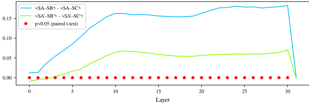
Average Difference in Cosine Similarity for Bio-Medical-Llama
