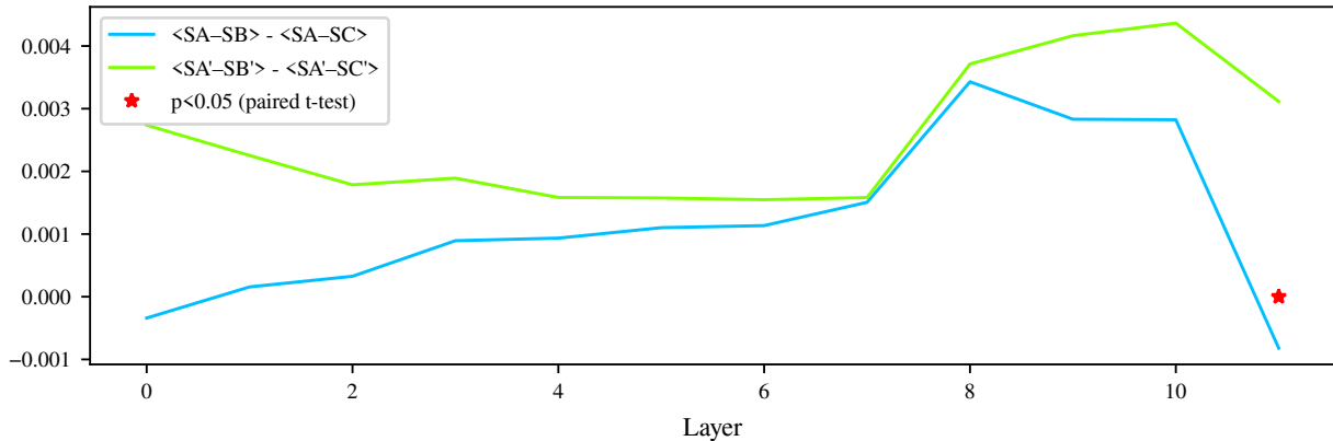
Average Difference in Cosine Similarity for FinanceBERT
