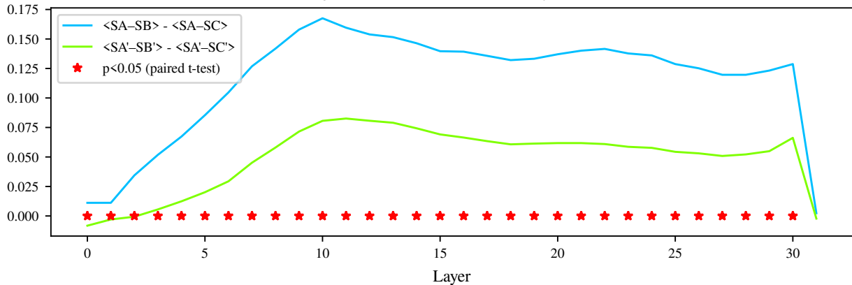
Average Difference in Cosine Similarity for Llama
