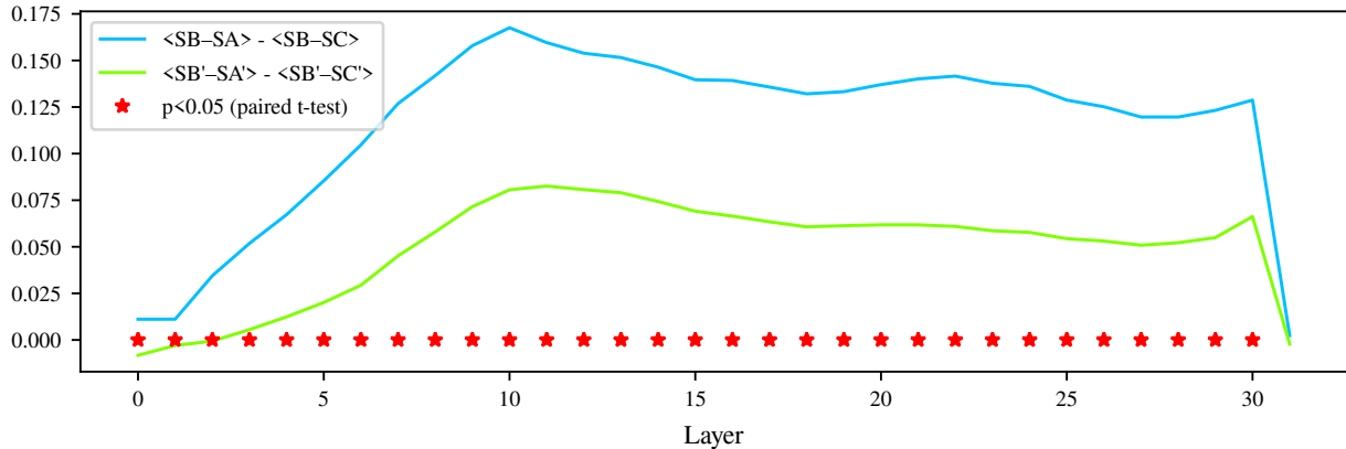
Average Cosine Similarity Difference for Llama
