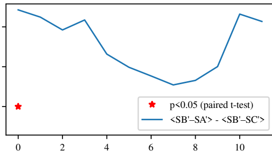
Primes
