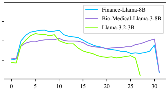
Euclidean Distance
