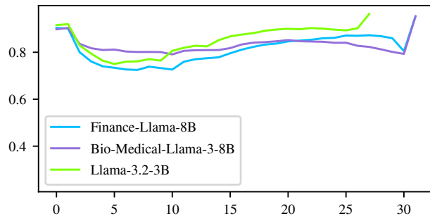
Cosine Similarity
