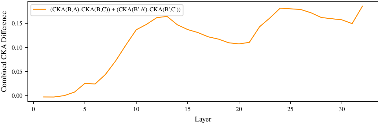
Combined CKA Difference for Bio-Medical-Llama-3-8B
